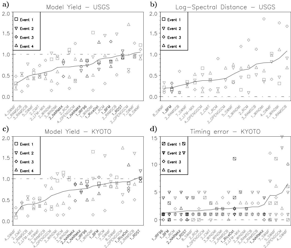
Figure 6. Model ranking using Yield (YI), Log-Spectral Distance M_s and Timing Error \Delta T . For YI in Panel a) and c) (USGS and Kyoto D_{st} , respectively), the best performing models are near the right (nearest the score of YI = 1 , shown as the dashed near the middle of the vertical range of each panel). Panel b) shows the log-spectral distance M_s based on USGS D_{st} with best-performing models on the left. For the Timing Error \Delta T , based on Kyoto D_{st} , in Panel d), Events 1 and 2 have been split and two values have been obtained. These values are indicated by the two squares with a diagonal line for Event 1 and two triangles with a vertical and horizontal line for Event 2. The best models (near \Delta T = 0 ) are on the left of the plot. Ideal scores ( M_s = 0 , \Delta T = 0 ) are shown as dashed lines near the bottom of the vertical ranges in both panels.
