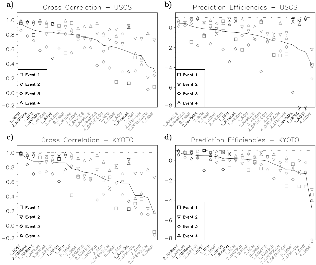
Figure 5. Model ranking using Correlation Coefficient ( CC ) and Prediction Efficiency ( PE ). Panel a) and c) show the ranking with respect to CC for USGS and Kyoto D_{st} , respectively. Models performing best on average are to the left. Besides the average score (solid line), the scores for the events are plotted as symbols for each run: Event 1: square, Event 2: triangle with point down, Event 3: diamond, and Event 4: triangle with point up. Panels b) and d) show the models ranked by Prediction Efficiency. Runs performed with the different model types are shown in different colors (magnetosphere models in red, ring current models in blue and D_{st} -specification models in black). All panels also contain the ideal score ( CC = 1 , PE = 1 ) as the horizontal dashed line near the top. Note that the vertical range for CC starts at -0.2 and ends at 1.1 and for PE the range starts at -8 and ends at 1.5. Two PE scores for 1_IRF96 (-10.6) and 1_RDST (-12.5) lie below the vertical plot range in Panel b) and one score for 4_SWMF (-9.1) is below the plot range in Panel d), indicated by the symbols with downward arrows at the bottom.
