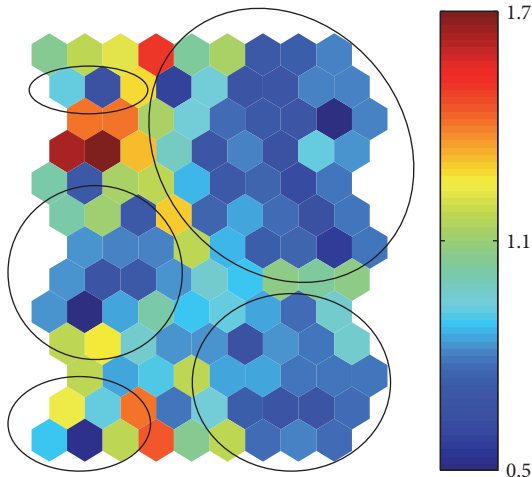
FIGURE 3: U-matrix of the 54 ERCs texts preprocessed through the VSM. Color scale is related to distances between map units. Red colors represent large distances and blue colors represent small distances.
