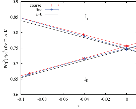
Figure 7: Form factors in z -space.
