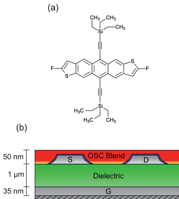
Fig. 1 (a) Chemical structure of 2,8-difluoro-5,11-bis(triethylsilyl)ethynylantradithiophene (diF-TES-ADT). (b) Schematic cross section of the bottom gate, bottom contact (BGBC) device architecture.
