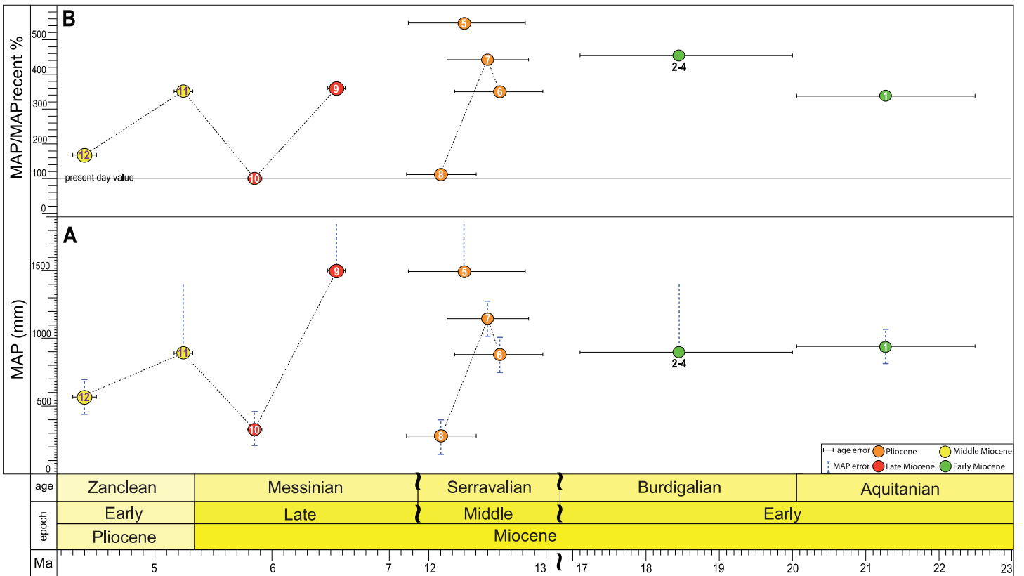
Figure 10 Palaeoprecipitation development of Western Siberia including the Zaisan Basin. (A) Curve displaying the development of the absolute values of mean annual precipitation (MAP); (B) the ratio of MAP to recent precipitation value (MAP/MAPrecent100%), dashed black line (100%) indicates the recent precipitation values. Localities: 1, Ayakoz; 2, Vympel; 3, Poltinik; 4, Tri Bogatyrya; 5, Kentyubek; 6, Malyi Kalkaman 2; 7, Malyi Kalkaman 1; 8, Baikadam; 9, Novaya Stanitsa 1A; 10, Cherlak; 11, Detskaya zheleznaya doroga; 12, Olkhovka 1B.
