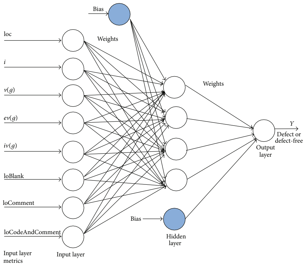
FIGURE 4: The proposed RBFNN model for JMI dataset.
