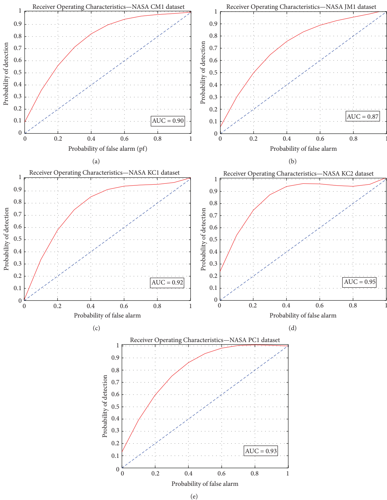
FIGURE 5: Receiver Operating Characteristics curve for five NASA datasets: (a) CM1, (b) JM1, (c) KC1, (d) KC2, and (e) PC1.
