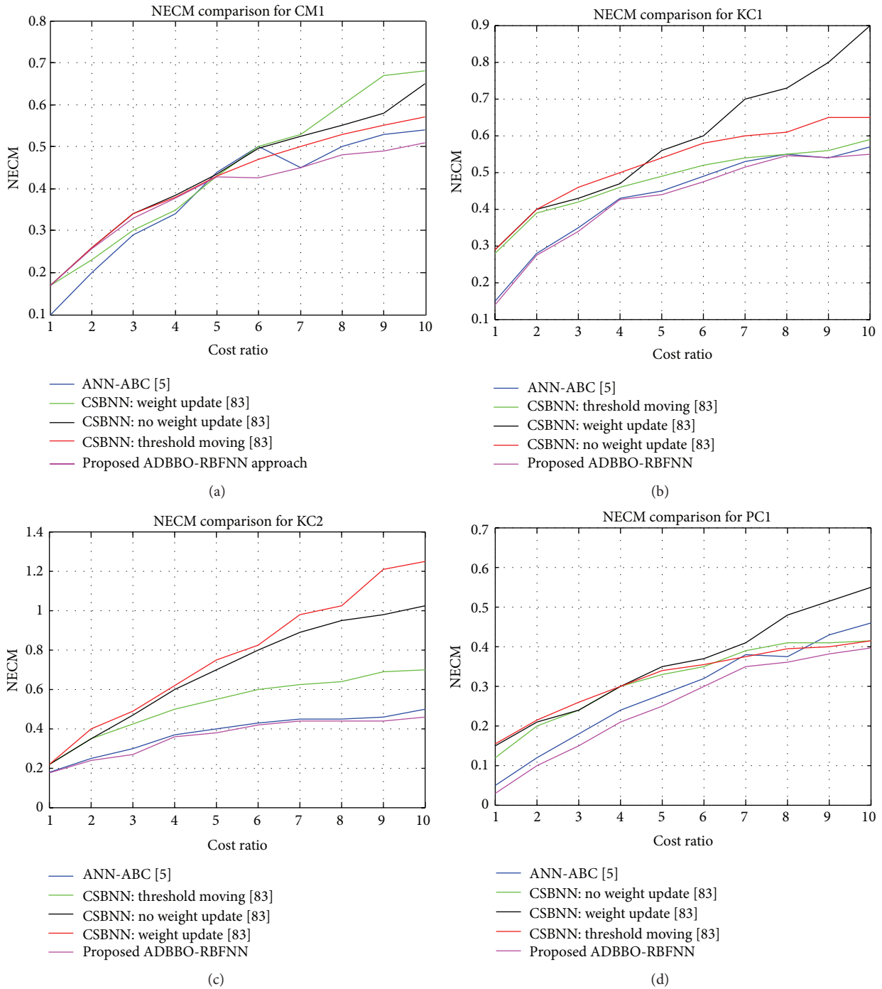
FIGURE 6: Cost ratio versus NECM comparison of the proposed model with other classifiers for NASA datasets (a) CMI, (b) KC1, (c) KC2, and (d) PCI.
