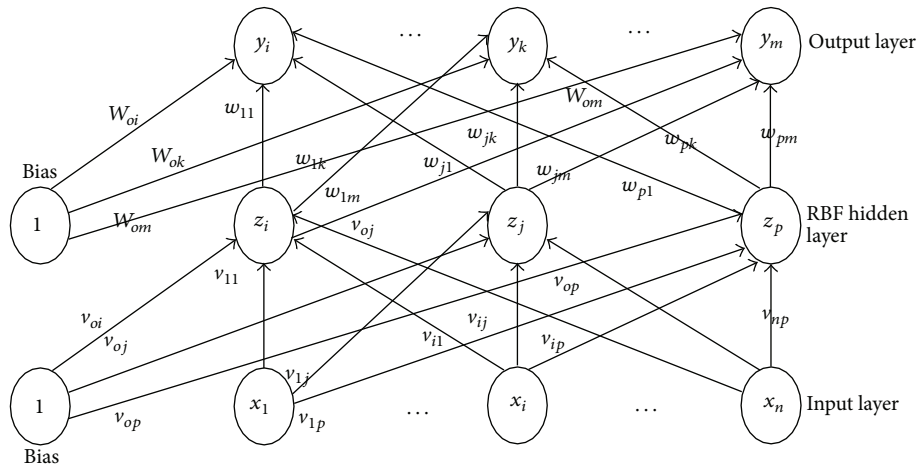
FIGURE 2: Architecture of radial basis function neural network model.
