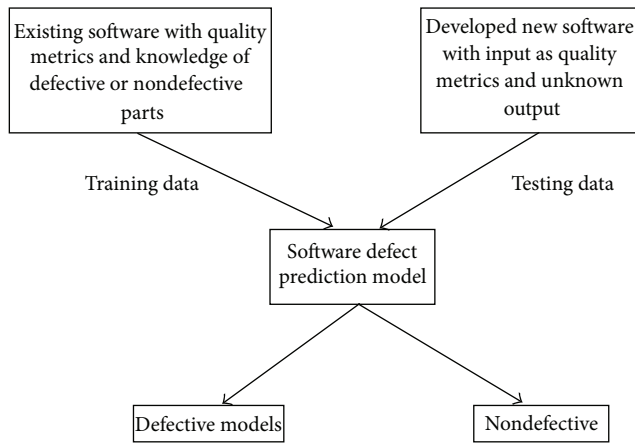
FIGURE 1: Basic software defect prediction model.
