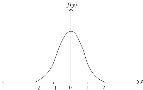
FIGURE 3: Gaussian activation function in RBFNN model.
