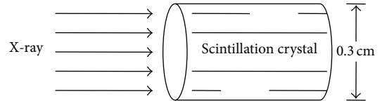
FIGURE 2: The Monte Carlo simulation model in our study.
