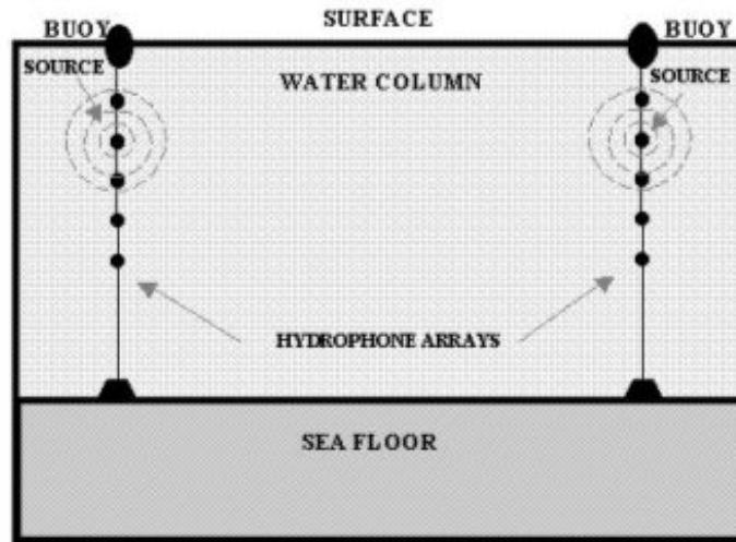
Figure 3.3 An optimum configuration of moorings for ocean acoustic tomography observatories.
