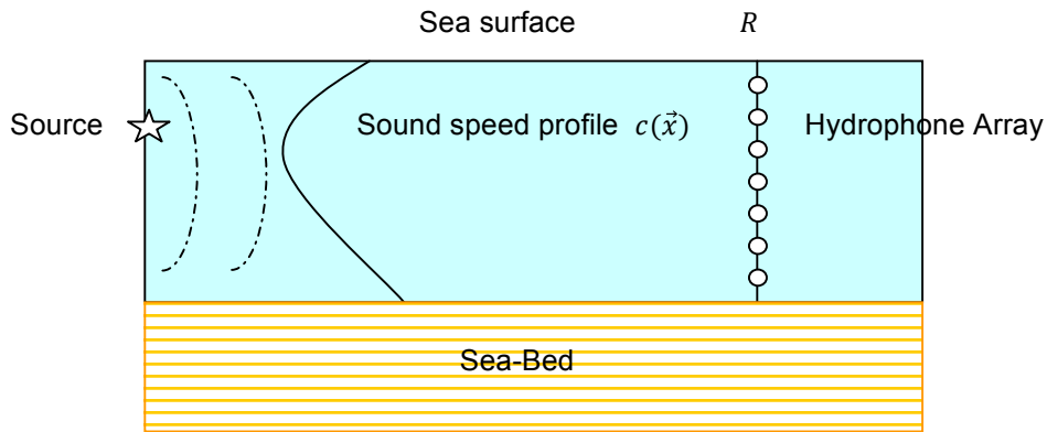
Figure 3.2 A vertical slice defined by a pair of transceivers in observatories for ocean acoustic tomography. Simplified version with horizontal plane water-bottom interface.
