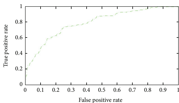
FIGURE 7: ROC curves of the SVM-based method for pupylation site prediction; the AUC value was 0.791.
