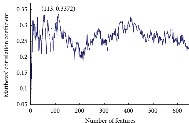
FIGURE 1: The IFS curve showed the values of MCC against feature numbers based on the data in Supporting Information Text S2. The maximum MCC was 0.3372 when 113 features were used. These 113 features were considered as the optimal feature set of our classifier.
