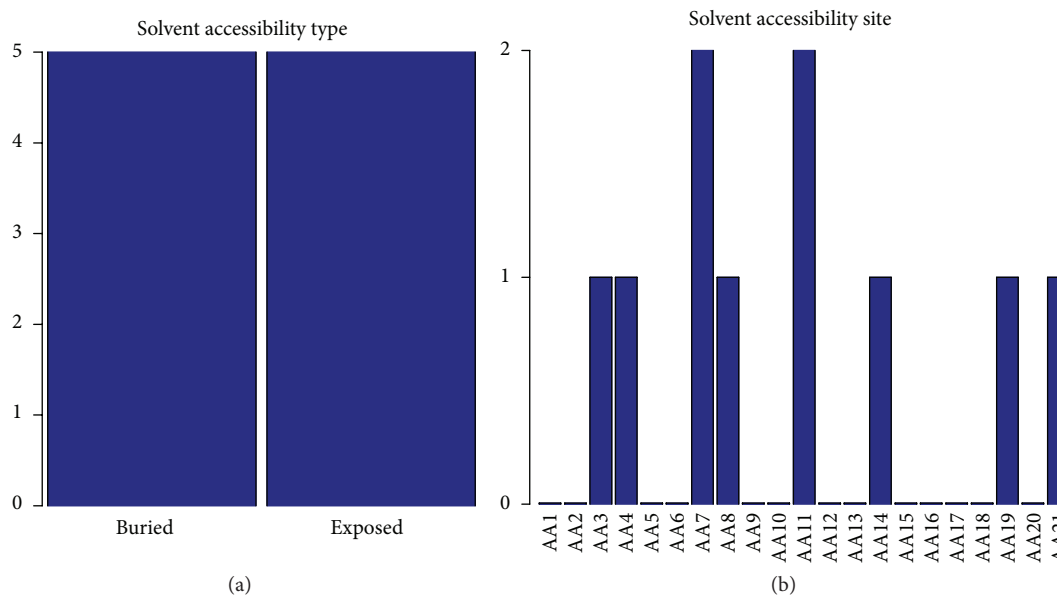
FIGURE 5: The number of each type or each site of solvent accessibility features in the optimal feature set. (a) The number of two types of solvent accessibility features (buried and exposed) in the optimal feature set. (b) The number of each site of solvent accessibility features in the optimal feature set.
