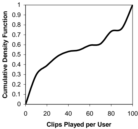
Figure 4. Cumulative Density Function (CDF) of Video Clips Played per User
