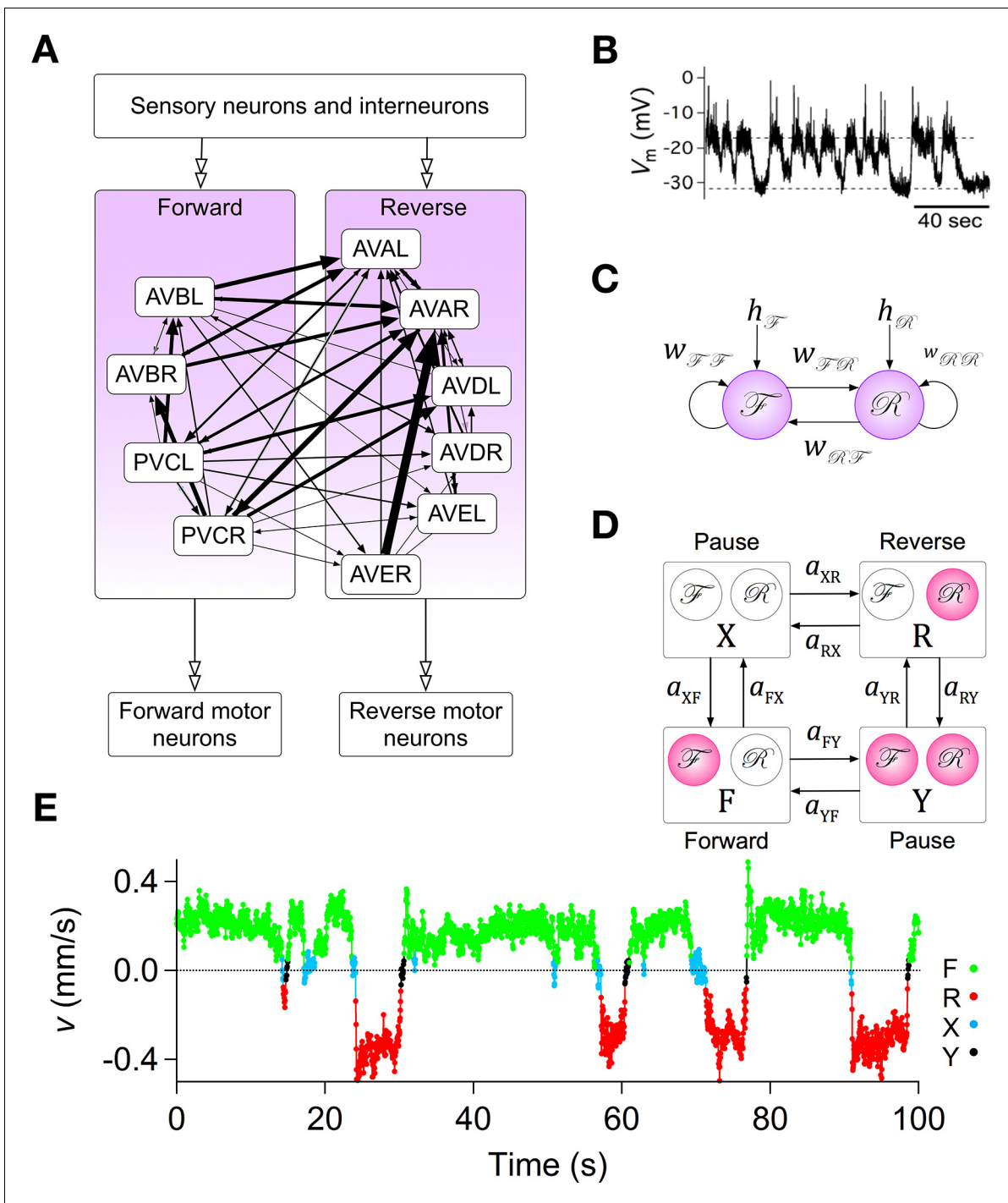
Figure 2. Assumptions with supporting data for the Stochastic Switch Model. (A) Connectivity of forward and reverse command neurons. Arrows with single heads are monosynaptic connections inferred from the C. elegans connectome (White et al., 1986; Varshney et al., 2011) line thickness is proportional to the number of presynaptic specializations seen in the reconstruction of each pairwise connection. Open, double-headed arrows indicate synaptic pathways from or to the indicated pool of neurons outside the network. (B) Voltage recording from the command neuron AVA in the absence of injected current. In this neuron, quasi-stable membrane potentials are seen at -17 and -32 mV. These results differ from previously published AVA recordings, which were made in the presence of hyperpolarizing current (5–10 pA) that kept the membrane potential near -55 mV (Lindsay et al., 2011). (C) Neuronal representation of the Stochastic Switch Model. Forward and reverse command neurons are represented as single binary neuron-like units \mathcal{F} and \mathcal{R} , respectively. Arrows depicting cross connections ( w_{\mathcal{F}\mathcal{R}}, w_{\mathcal{R}\mathcal{F}} ) represent functional (net mono- and polysynaptic) connections between forward and reverse units. Self-connections ( w_{\mathcal{F}\mathcal{F}}, w_{\mathcal{R}\mathcal{R}} ) represent synaptic connections between neurons comprising a given unit, voltage dependent currents in these neurons, and polysynaptic recurrent pathways involving non-command neurons. Downward arrows ( h_{\mathcal{F}}, h_{\mathcal{R}} ) represent the Figure 2 continued on next page
