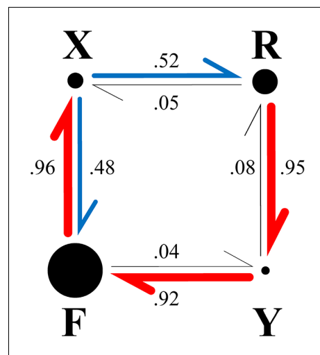
Figure 3. Fate diagram of the model. The system typically cycles clockwise through states F, X, R, Y, with state F frequently interrupted by FXF transitions, leading to state sequences of the form \dots(FX)_nRY(FX)_nRY\dots . Nearly unidirectional transitions out of a given state are shown by red arrows; blue arrows indicate nearly equiprobable transitions. The width of the arrows and the numbers beside them show the probability that the transition out of the state at the tail of the arrow is into the state at the head. The area of each circle is proportional to the probability of the corresponding state ( Table 1 , column A).
