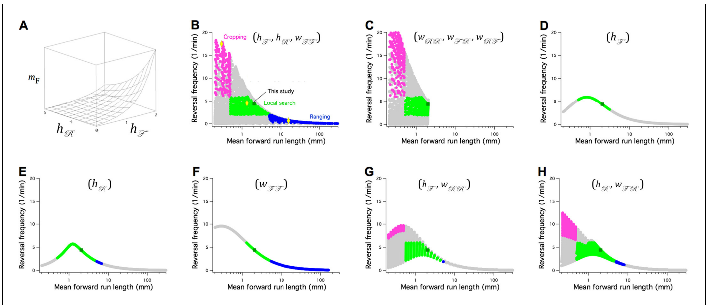
Figure 8. The Stochastic Switch Model accounts for the three main modes of random search in C. elegans . (A) Plot of mean forward run length versus the weights h_{\mathcal{F}} and h_{\mathcal{R}} , illustrating a minimal model of search-scale regulation. (B-H) Calculated effects on search mode of the weights indicated in parentheses. The frequency of reversals ( f_{FPR} ) is plotted against m_F while these three weights are scanned from -6 to 6 weight units in steps of 0.4. Each point was categorized as cropping (magenta), local search (green), ranging (blue), or indeterminate (grey) according to value of f_{FPR} and m_F , and whether or not the associated value of m_R (not shown) indicated a short or long reversal; see Materials and methods for definitions of search modes. Yellow diamonds mark the scanned points modeled in Figure 8—figure supplement 1. A = 1 Hz; similar results were obtained for A = A_{max} and A = A_{min} (Table 7).
