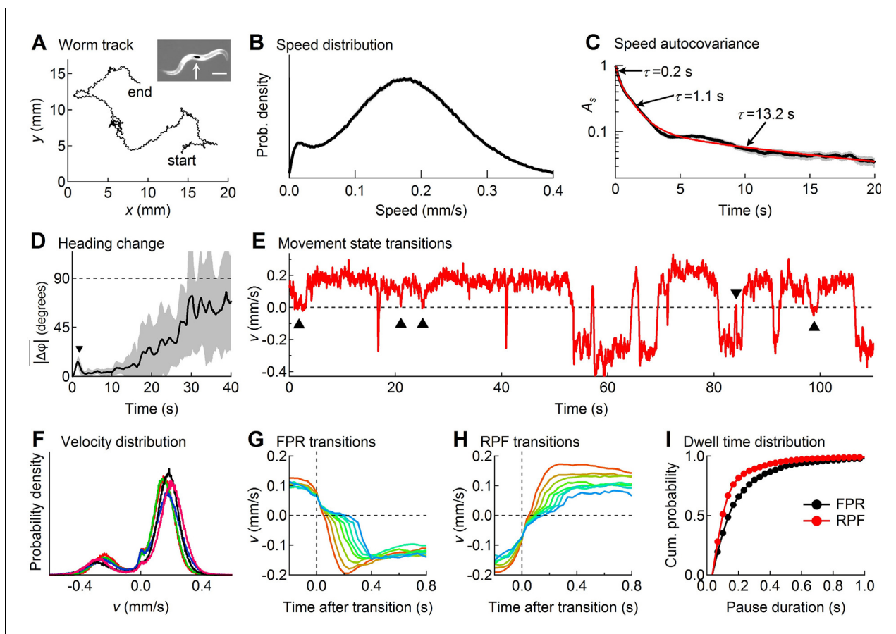
Figure 1. Descriptive statistics of wild type worm tracks. (A) (x, y) -coordinates of a worm during 10 min of foraging. Inset: Image of a worm showing the black spot (arrow) used for optical tracking (scale bar = 200 \mu\text{m} ). (B) The speed distribution computed from the distance moved between successive video frames had a peak at 180 \mu\text{m/s} , which includes both forward and reverse locomotion. A second peak at 14 \mu\text{m/s} corresponds to pauses. The decreased probability of observing speeds <14 \mu\text{m/s} ( <0.47 \mu\text{m/frame} ) is due to noise in the position measurement. (C) At least three time constants were required to fit (red) the speed autocovariance function (black; grey shading shows \pm 1 sem). (D) The worm's heading remained nearly constant for \sim 10 s except for a transient peak at 1.4 s ( \blacktriangledown ), which corresponds to the period of one half cycle of undulation during sinusoidal locomotion. The dashed line shows random reorientation; shading shows \pm 1 sem. (E) Example of v(t) showing periods of forward locomotion, reverse locomotion and pauses of various durations. Upward triangles ( \blacktriangle ) mark forward-pause-forward (FPF) events; the downward triangle ( \blacktriangledown ) marks a reverse-pause-reverse (RPR) event. (F) Velocity distributions for the 5 wild type cohorts (5 colors) analyzed in this study. (G) Ensemble-averaged velocity during FPR transitions. All FPR transitions in all wild type cohorts were aligned at the end of forward movement, grouped according to the duration of the pause (2–9 frames), and averaged. Such transitions were defined using a threshold criterion of |v| < 50 \mu\text{m/s} to identify state P (Rakowski et al., 2013). Pauses lasting \leq 1 frame are not shown because of ambiguity in state identification; pauses lasting \geq 10 frames are omitted for clarity. (H) Identical to G except RPF transitions are shown. (I) Cumulative probability distributions for dwell time in the pause state defined as in G and H for all FPR and RPF transitions of duration >1 frame in wild type worms.
