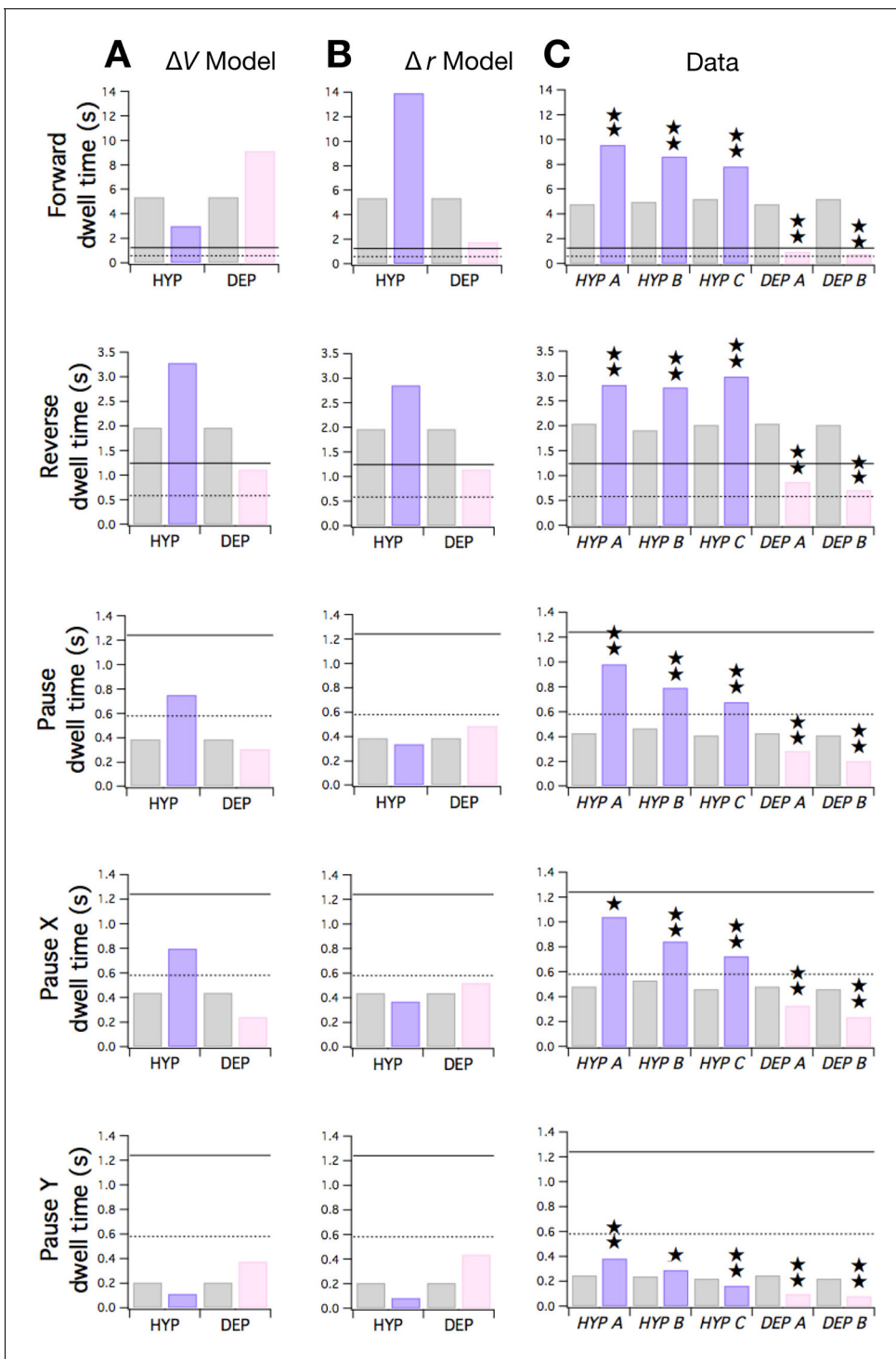
Figure 7. Predicted and observed effects of HYP and DEP mutations on dwell times. (A) Predicted effects of changes in membrane potential. (B) Predicted effects of changes in input resistance. (C) Dwell times in F, R, and P for cohorts of HYP mutants, DEP mutants, and wild type animals. Stars indicate significant change in dwell time ( p < 0.05 without (★) or with (★★) correction for multiple comparisons; Table 6 ). In A-C wild type dwell times are indicated by gray bars. Horizontal lines indicate the estimated range of d_0 , the dwell time in the uncoupled state. In the \Delta V model, h terms were made more negative to model HYP mutants and more positive to model DEP mutants by subtracting or adding a constant \Delta h = 0.6 ; qualitatively similar results were obtained for 0 < \Delta h \leq 0.8 . In the \Delta r model, h and w terms were scaled by (1 + f) to model HYP mutants and by (1 - f) to model DEP mutants, with f = 0.6 ; qualitatively similar results were obtained for 0 < f \leq 1 . Strains, HYP A: DA572 eat-4(ad572) ; HYP B: MT6308 eat-4(ky5) ; HYP C: KP4 glr-1(n2461) ; DEP A: VM1136 lin-15(n765); akIs9 [lin-15(+), Pglr-1::GLR-1(A/T)] ; DEP B: VM188 lin-15(n765); akEx52[lin-15(+), Pnmr-1::GLR-1(A/T)] . DOI: 10.7554/eLife.12572.023
