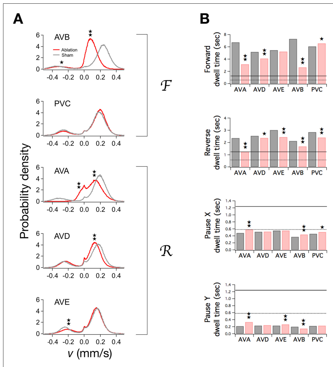
Figure 5. Ablation of command neurons. (A) Velocity distribution of ablated cohorts (red) compared to sham operated controls (grey) when the indicated command neuron was killed. Stars indicate significant reduction in velocity for the indicated peak ( p < 0.05 without (★) or with (★★) correction for multiple comparisons; Table 3 ). (B) Dwell times in F, R, and P in ablated (red) and sham operated animals (grey). Stars indicate significant differences from sham (as defined in Table 4 ). Horizontal lines indicate the estimated range of d_0 , the dwell time in the uncoupled state. Each group of ablated animals was tested in parallel with a distinct set of sham operated controls to minimize the effects of variation between populations. Error bars for dwell times are not shown because statistical significance was calculated using the likelihood ratio test (see Table 4 legend), which does not generate sem estimates, and calculation of confidence intervals would have required an excessive amount of computation time. Stars indicate p < 0.05 without (★) or with (★★) correction for multiple comparisons ( Table 4 ). DOI: 10.7554/eLife.12572.017
