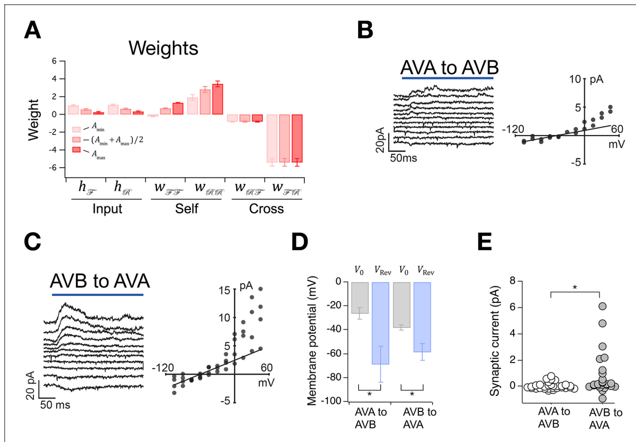
Figure 6. The Stochastic Switch Model correctly predicts the sign and strength of synaptic connections. (A) Synaptic weights (mean \pm sem, n = 5 cohorts) from maximum likelihood fits to velocity data from wild type worms. (B, C) Left , synaptic current in AVB or AVA when the indicated presynaptic neuron was photoactivated (blue line). Right , mean synaptic current during the first 100 ms of the stimulus plotted against holding potential in the postsynaptic neuron ( I - V curve). Lines show linear fits to the data at negative holding potentials which were used to estimate v_{Rev} . (D), Zero-current holding potential and reversal potential of synaptic currents (mean \pm sem) in the indicated postsynaptic neuron (paired t -tests: AVA to AVB, p = 0.043 , n = 9 ; AVB to AVA, p = 0.019 , n = 17 ). (E), Scatter plot of synaptic currents recorded at a holding potential of -15 mV (unpaired t -test: p = 0.010 , n \geq 25 ). DOI: 10.7554/eLife.12572.021
