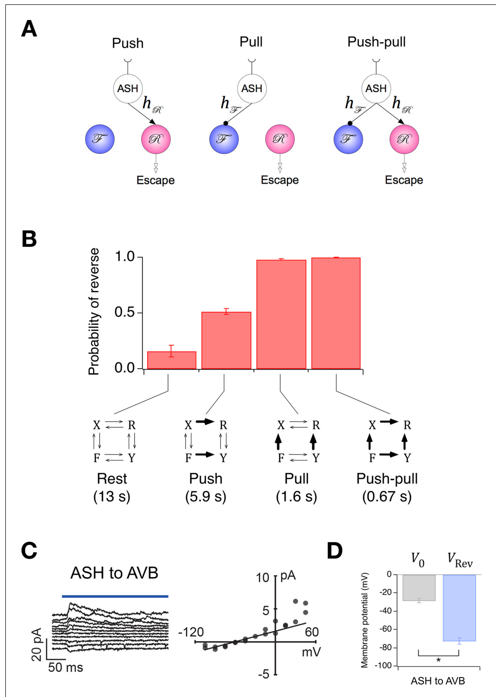
Figure 9. Extension of the Stochastic Switch Model to deterministic behaviors. (A) Three functional circuit motifs for deterministic escape behavior initiated by the nociceptive neuron ASH. (B) Predicted steady-state probability of reversal behavior in the resting state and the activated state of the three motifs shown in A. Plotted values are means across the five wild type cohorts shown in Figure 1F. Error bars are \pm sem. Numbers in parenthesis are predicted mean first latency to a reversal response. (C) Left, synaptic current in AVB when ASH was photoactivated (blue line). Right, mean synaptic current during the first 100 ms of the stimulus plotted against holding potential in AVB. The line is fit to the data at negative holding potentials. (D) Mean zero-current holding potential and mean reversal potential of synaptic currents ( \pm sem) in AVB (paired t -test: p=0.013 , n=4 ).
