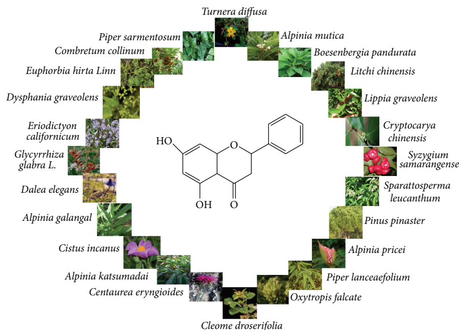
FIGURE I: Chemical structure and natural sources of pinocembrin.
