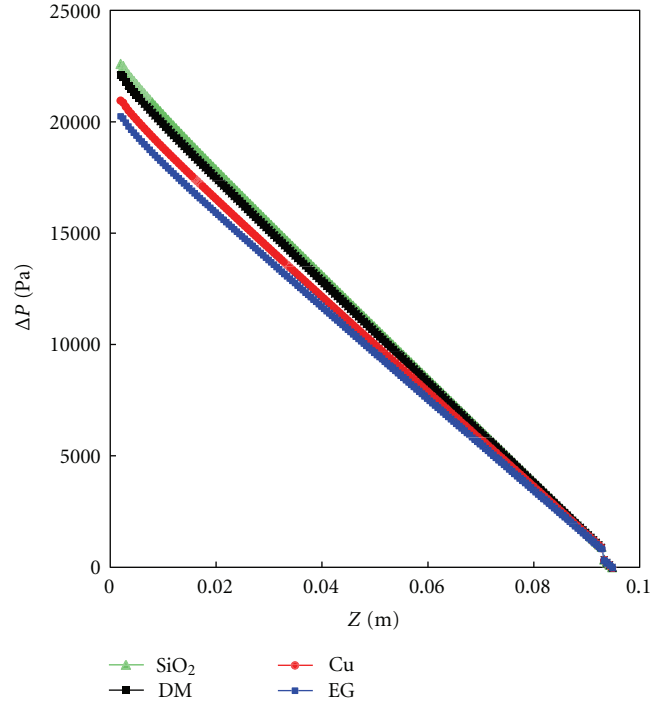
FIGURE 7: Pressure distribution along the tube length.
