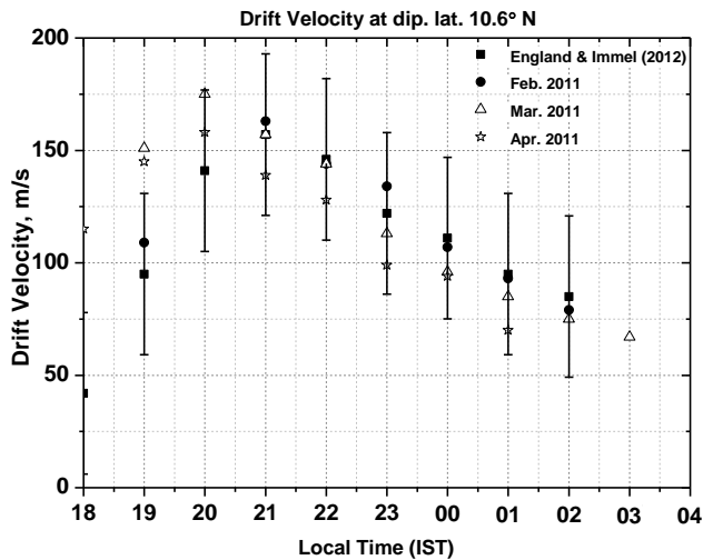
Fig. 7. The monthly mean zonal drift velocities of EPBs compared with values of the empirical model for the months of February, March and April 2011.
