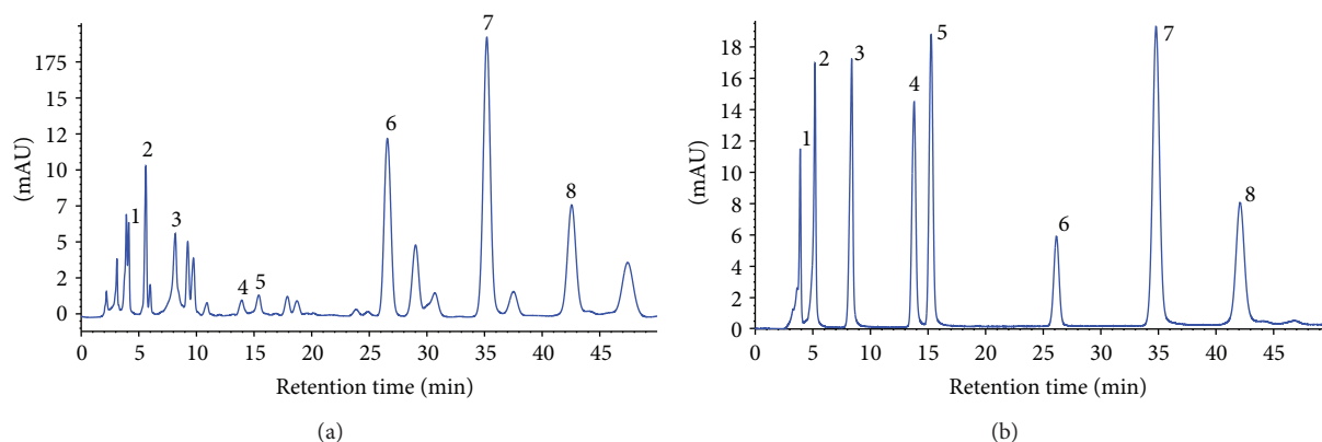
FIGURE 1: HPLC chromatogram of (a) EECP and (b) flavonoids standards. Peaks: (1) rutin; (2) myricetin; (3) quercetin; (4) kaempferol; (5) apigenin; (6) pinocembrin; (7) chrysin; and (8) galangin.
