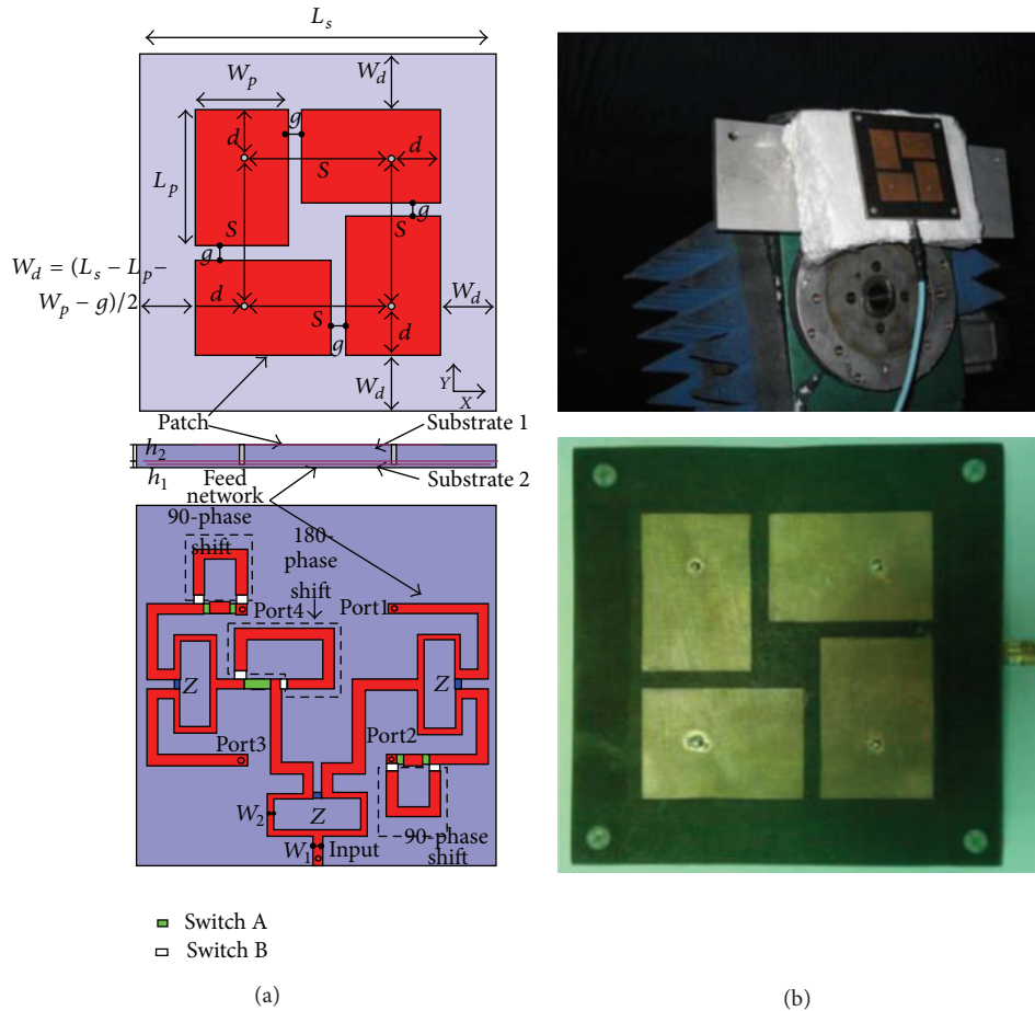
FIGURE 11: (a) The pattern and polarization reconfigurable microstrip antenna. (top) Top view. (middle) Side view. (bottom) Bottom view. (b) Measurement setup photograph and the fabricated antenna (with permission from IEEE).
