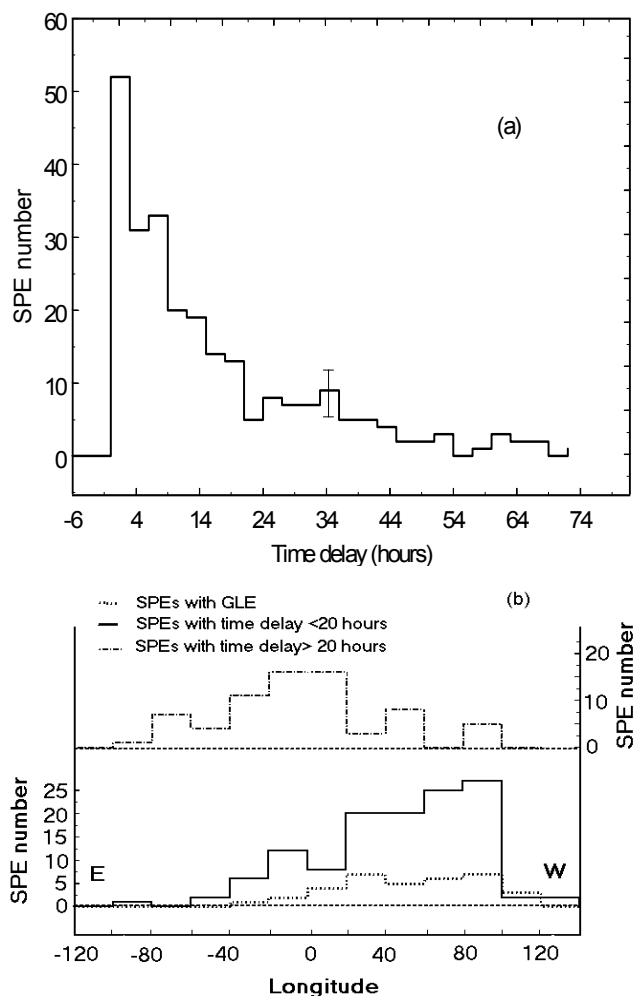
Fig. 7. (a) The SPEs number with respect the time delay between the proton event maximum and the onset time of the Ha “associated flares” is presented. (b) The longitudinal distribution of the SPEs in three cases (with GLE, with time delay <20 h and with time delay >20 h) is also illustrated.
