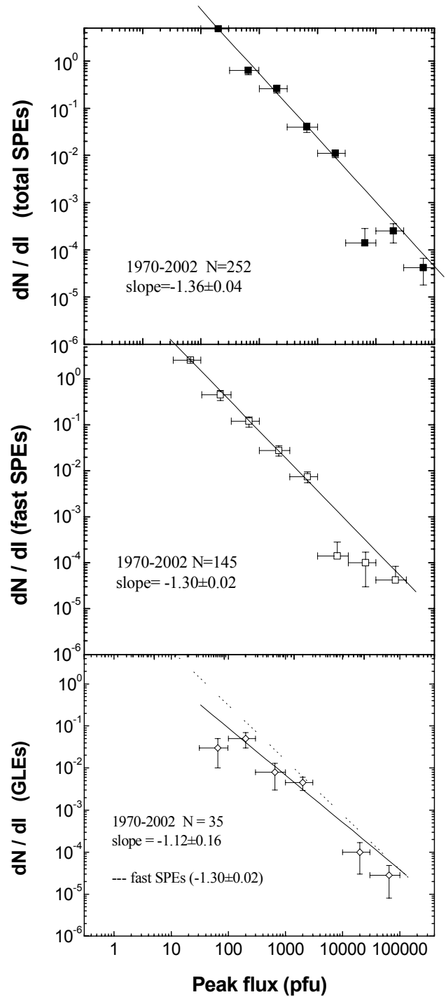
Fig. 8. Peak size distributions of the total number of SPEs with energies E>10 MeV (upper panel), of the fast SPEs (middle panel) and of the SPEs connected with GLEs (lower panel) that appeared.
