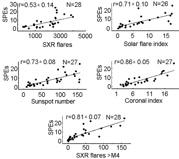
Fig. 4. Scatter plots and linear approximations of SPEs yearly number dependences on the total SXR flares, sunspot number, solar flare index, coronal index and SXR flares with importance >M4.
