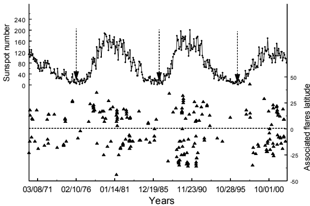
Fig. 5. “Butterfly diagram” of the associated with SPEs flares for the interval 1970–2002 is presented in the lower curve. Time profile of the sunspot number is also given in the upper curve.
