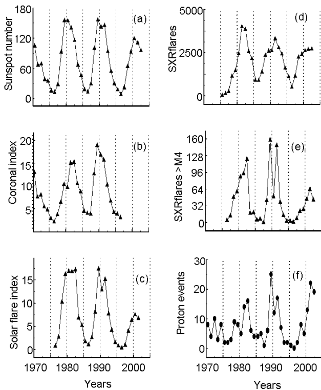
Fig. 2. Time distributions of the yearly values of (a) sunspot number, (b) coronal index, (c) solar flare index, (d) SXR flares number, (e) SXR flares number with importance > M4 and (f) proton event number with E > 10 MeV and peak intensity > 10 pfu, during the time interval 1970–2002.
