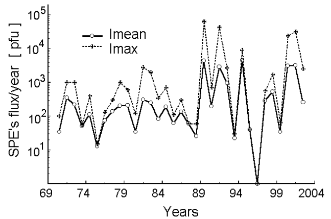
Fig. 3. Time distribution of yearly averaged and maximum intensity of the SPEs flux from 1970 to 2002.
