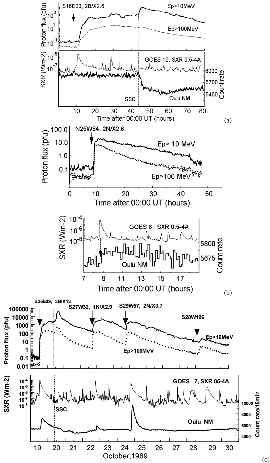
Fig. 1. Typical examples of large solar proton events which occurred on 24 September 2001, 25 July 1989 and during the time interval from 18 October to 31 October 1989, respectively.
