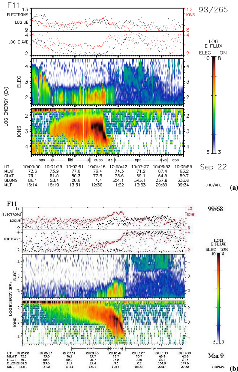
Fig. 2. DMSF F11 spectrograms of differential energy flux ( \text{eV}/\text{cm}^2 \text{ s str} ). Top two line plots show total energy flux ( \text{eV}/\text{cm}^2 \text{ s str} ) and average energy (eV) of ions (red) and electrons (black). Cusp particle precipitation was observed at the time of (a) 10:03–10:04 UT on 22 September 1998 and (b) 09:10–09:11 UT on 9 March 1999.
