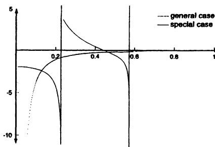
Fig.2. \sigma_\phi/A vs. r for t = 0.5
