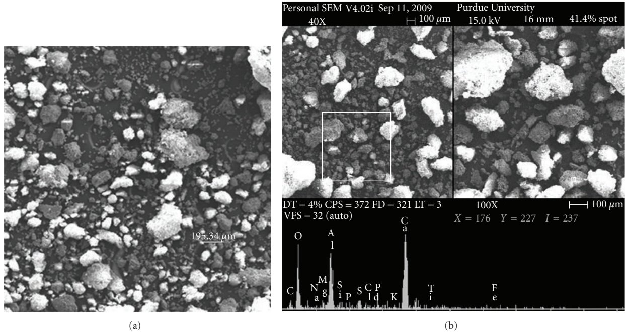
FIGURE 10: SEM micrographs of EAF(L) slag. (a) sand- and silt-size particle shapes (magnification = 50X) and (b) particles with their elemental analysis.
