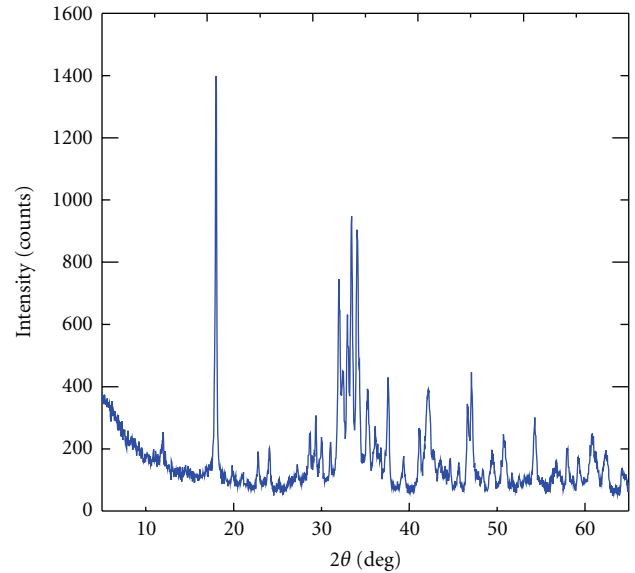
— BOF slag X-ray diffraction pattern
