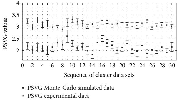
FIGURE 4: Trend of PSVG values calculated for a specimen set of 30 cluster data sets (both experimental and their MC simulated ones as shown in Tables 1 and 2) extracted from the visibility graph corresponding to one of the four data sets of \phi -values for ^{32}\text{S-AgBr} (200A GeV) interaction data (constructed in step (1)).
