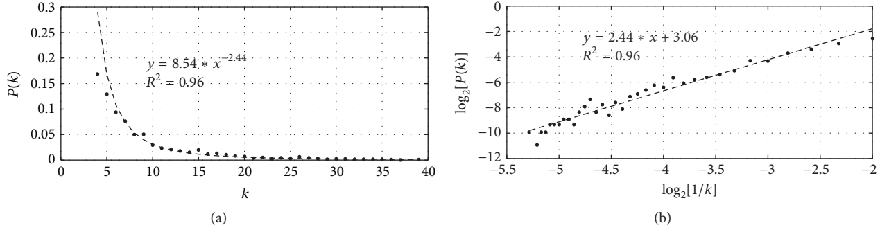
FIGURE 3: (a) P(k) versus k plot for a cluster (b) \log_2[P(k)] versus \log_2[1/k] plot for the same cluster.
