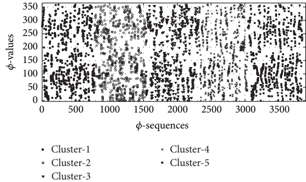
FIGURE 2: 5 clusters extracted from the azimuthal space corresponding to a sample pseudorapidity data set around c_r for ^{32}\text{S} -AgBr (200A GeV) interaction.
