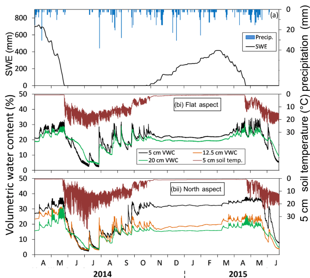
Figure 6. (a) Daily snow water equivalent (SWE) and precipitation recorded at the Dry Lake SNOTEL station and (b) the hourly soil volumetric water content (VWC) and 5 cm deep temperature at (bi) the flat SNOTEL site and (bii) the installed sensors on the north aspect slope.
