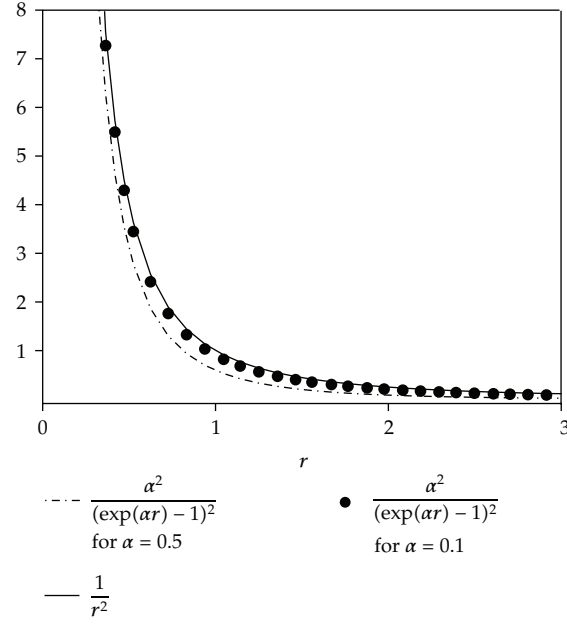
Figure 1: 1/r^2 and its approximation for different value of \alpha .
