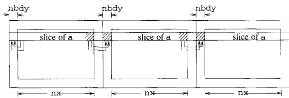
FIGURE 7 Fake and boundary zone updates for left side of grid.
