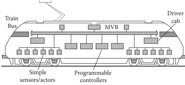
FIGURE 1: Multifunction Vehicle Bus in a locomotive.
