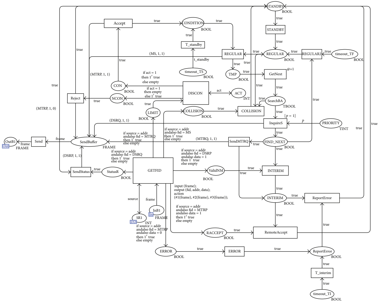
FIGURE 7: BusAdmin1 module.
