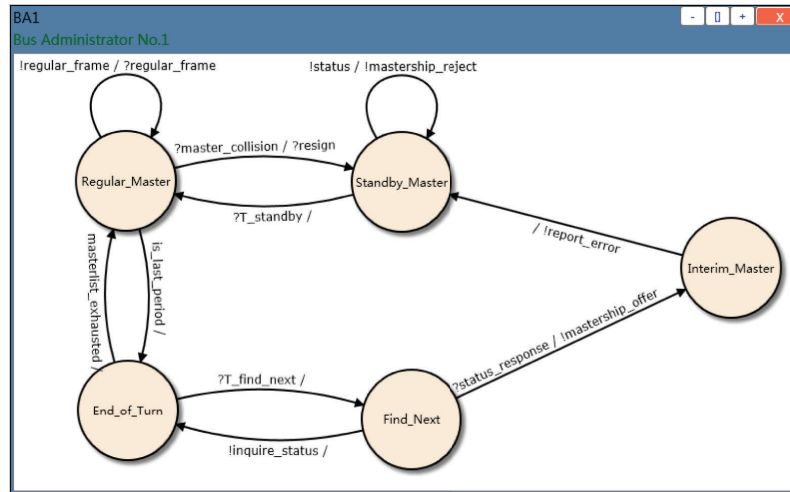
FIGURE 12: Model of a BusAdmin constructed in M 3 C.
