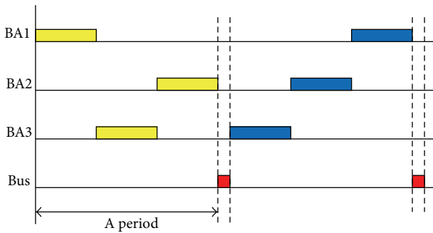
FIGURE 9: Timing diagram of the synchronous model.
