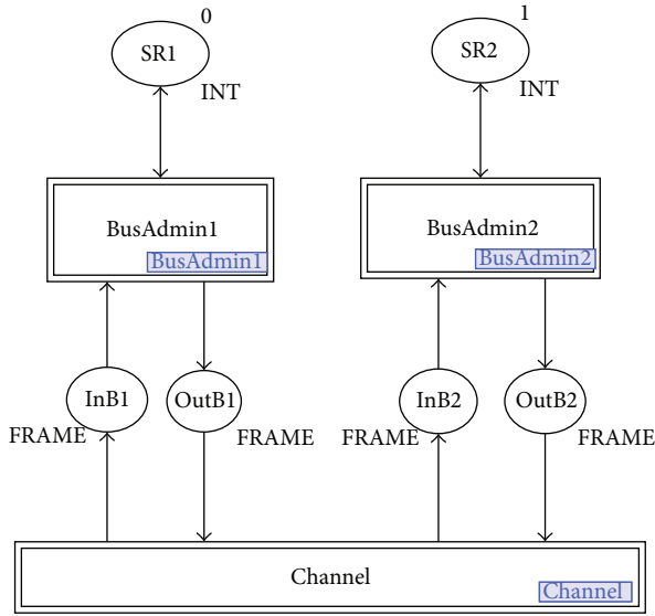
FIGURE 5: Top module.
