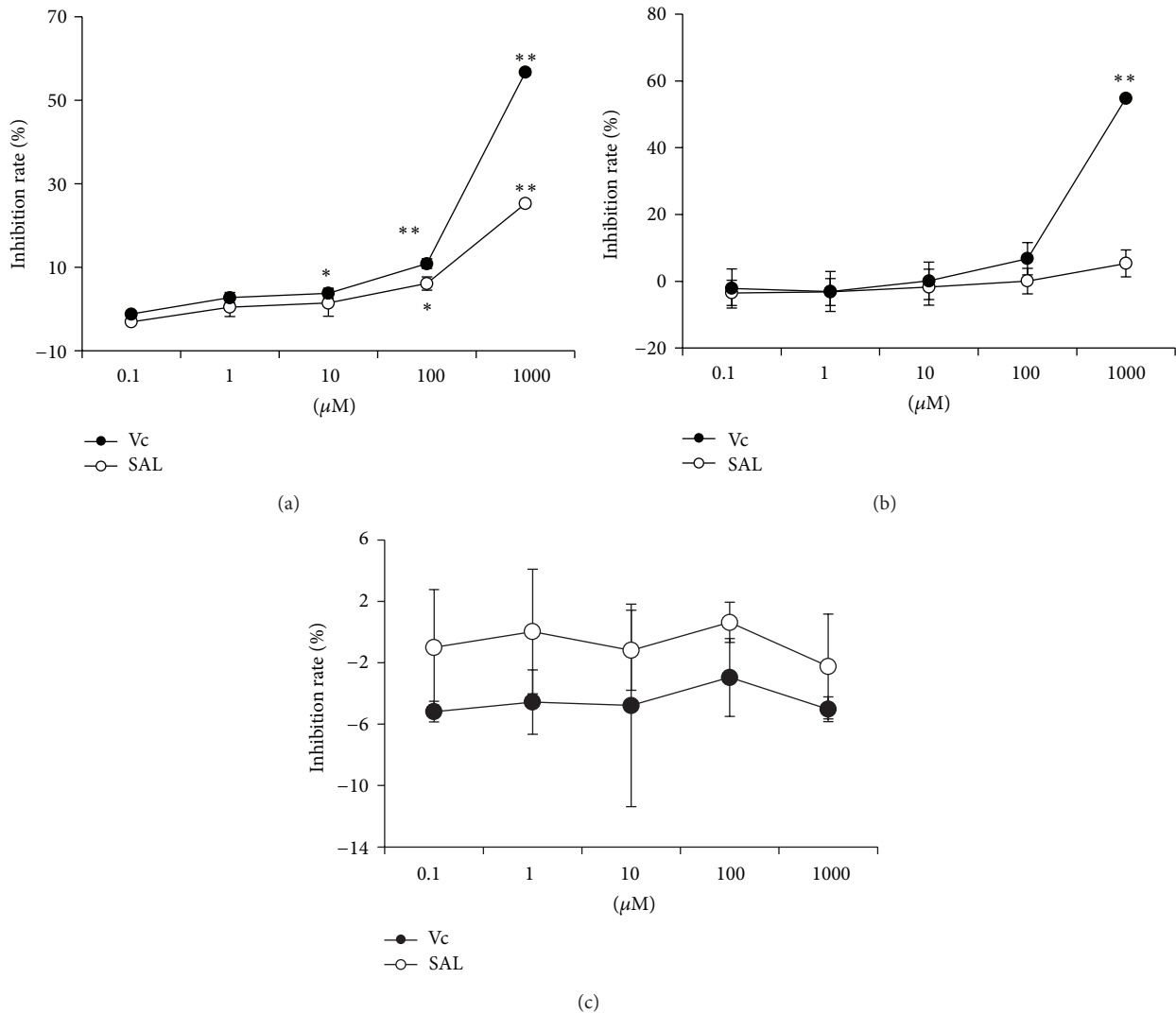
FIGURE 2: Effect of SAL on cell free ROS detection using different assay systems. (a) \text{OH}^\bullet was generated by Fenton reaction, (b) \text{O}_2^{\cdot-} was generated by xanthine/xanthine oxidase, and (c) \text{H}_2\text{O}_2 was exogenously added. * P < 0.05 , ** P < 0.01 versus blank control, n = 3 .
