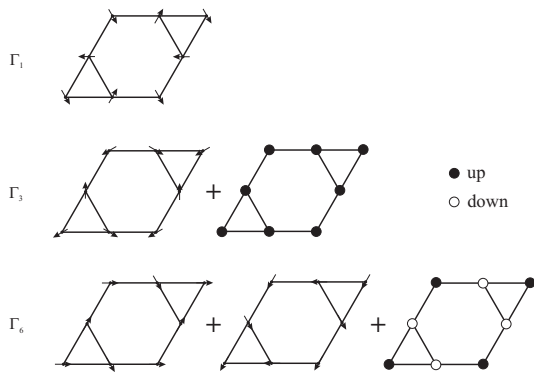
FIG. 5. The motifs for the different basis vectors for the non-zero irreducible representations of the point group D_{3d}^5 at the B site for the propagation vectors \mathbf{k}=0 and \mathbf{k}=00\frac{3}{2} . The labelling scheme follows that for \mathbf{k}=0 . 14
