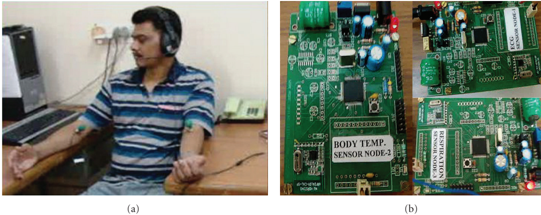
FIGURE 5: A patient's vital signs being recorded with three sensors measuring ECG, respiration and temperature.
