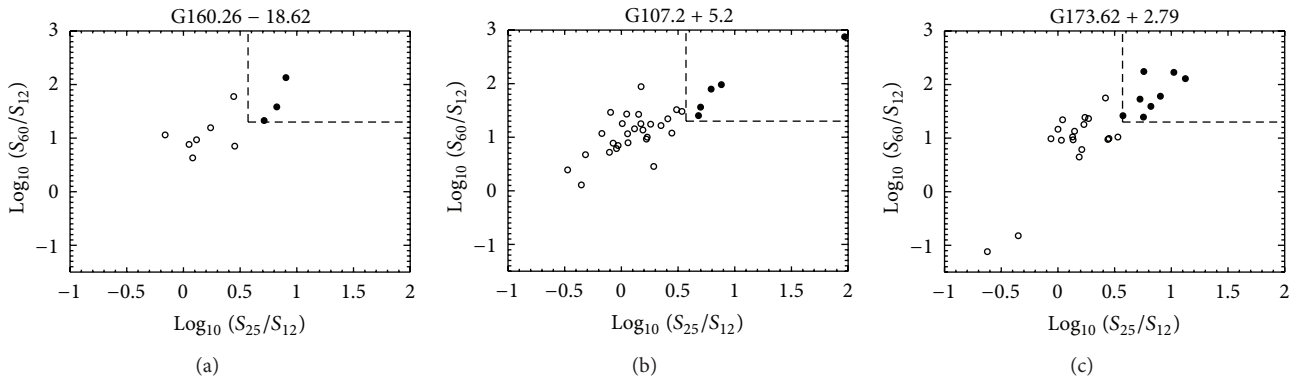
FIGURE 2: Colour-Colour plots of IRAS sources in the vicinity of Perseus (a), G107.2+5.2 (b), and G173.6 + 2.79 (c) AME regions. The colours are calculated for sources within 1^\circ of the central source positions using the IRAS PSC. UCHII region candidates, shown as solid-filled circles, have ratios \log_{10}(S_{60}/S_{12}) \geq 1.30 and \log_{10}(S_{25}/S_{12}) \geq 0.57 , corresponding to the top-right hand corner of this plot (marked with a dashed line).
