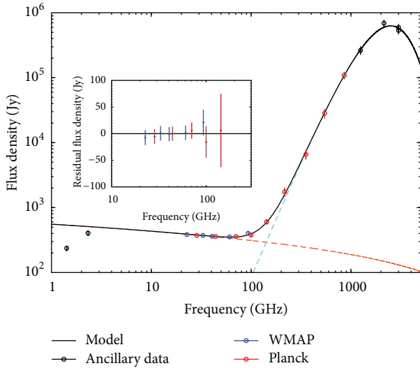
FIGURE 1: SED of the Orion Nebula (M42) HII region [4]. Free-free emission dominates at frequencies below 100 GHz while thermal dust emission dominates above 100 GHz. The free-free emission is optically thin above a few GHz. There is no evidence of significant AME.
