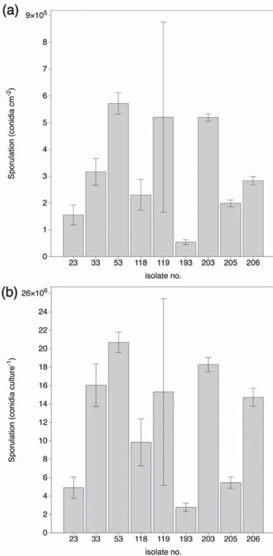
Fig. 3. Sporulation of B. bassiana isolates used for pathogenicity bioassays against RPW. a) Density of conidia (as conidia cm^{-2} ) of B. bassiana cultures on corn meal agar (CMA). b) Number of conidia per CMA 24-day culture of each isolate.
