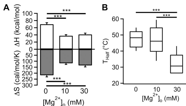
Figure 9. Thermodynamic analysis of Mg^{2+} effects on heat activation. (A) Measured \Delta H values (open bars) and \Delta S values (shaded bars) from heat-induced currents. Error bars indicate \pm SEM. (B) Box-and-whisker plot of the half-activation temperature T_{half} at the corresponding Mg^{2+} concentration. ***, P < 0.001 ; n = 5-6 .
