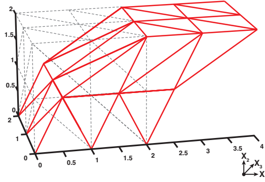
Figure 13: Deformed shape of “Not-so-simple” shear with Dirichlet boundary conditions.
