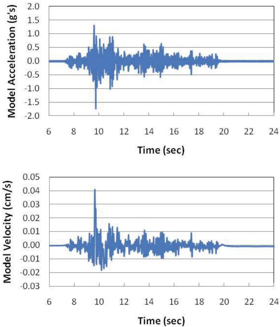
Figure 4. Model soil acceleration and velocity time histories in response to the table input earthquake motion CPM-000 (PGA=1.5g). Maximum horizontal acceleration occurs at t=9.61 s, the same time as the peak in velocity. For scale model similitude the time step is compressed ( \lambda^{0.5} ) to afford proper dynamic response on the shake table.
