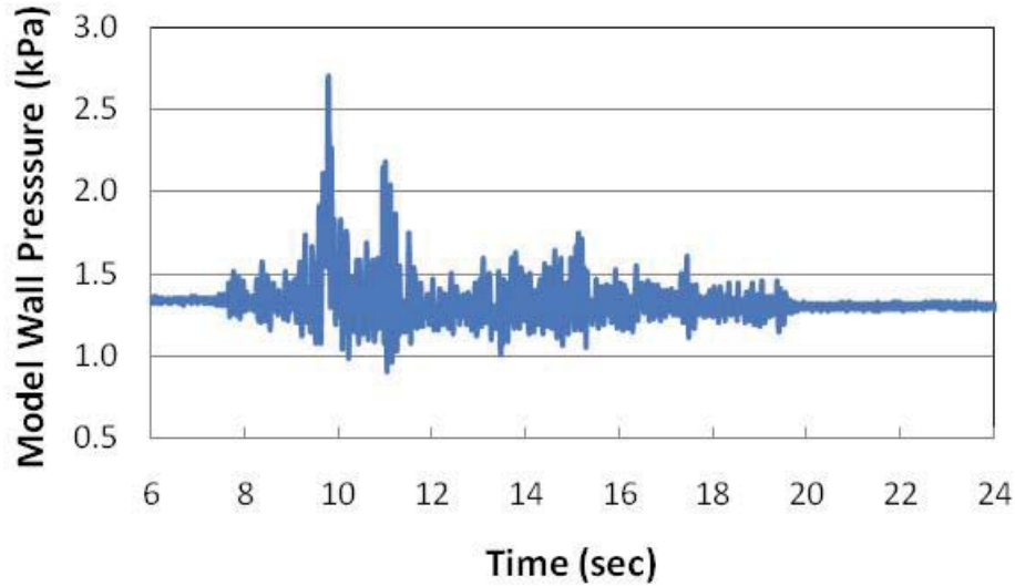
Figure 5. Model wall pressure time history in response to input table earthquake motion CPM-000 (PGA=1.5g). Maximum total scale model wall pressure, including the seismic increment, is P_{AE}=2.7 kPa at t=9.75 s. This is equivalent to 27 kPa in prototype scale as the scaling factor is \lambda=10 and pressure similitude is 1:\lambda .
