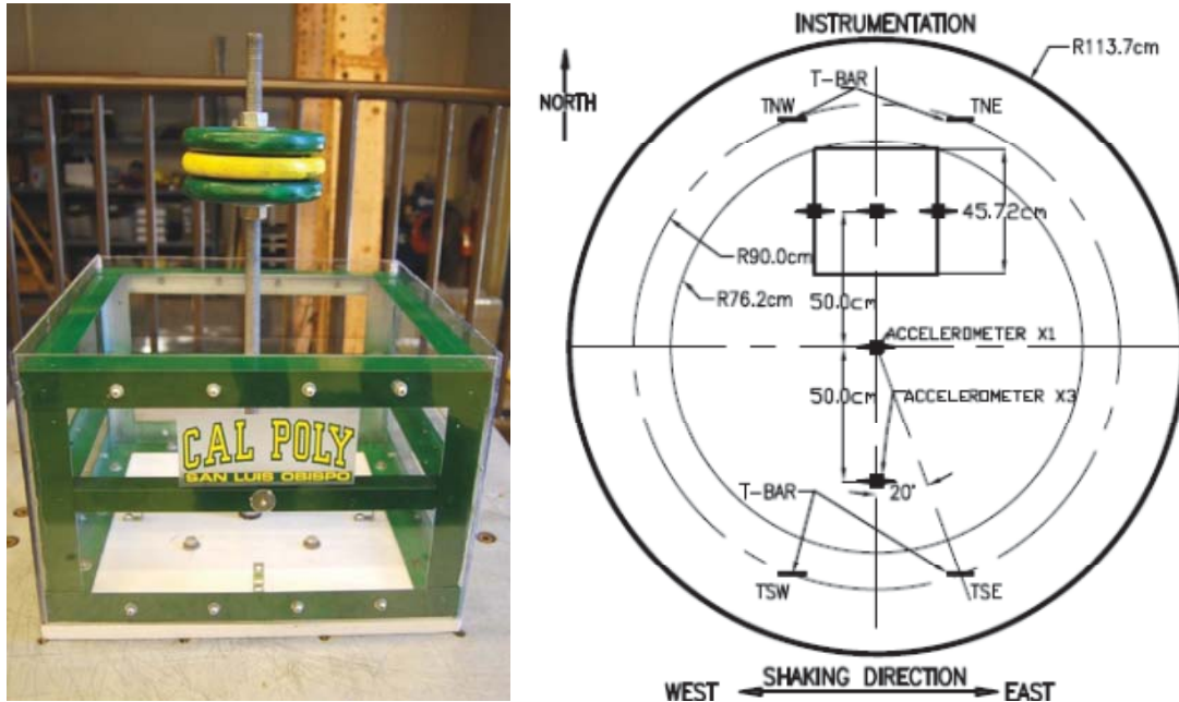
Figure 3. Picture (left) shows the scale model basement and retaining wall. The foundation is 46cm square, and the wall for this configuration is 32cm tall. The single degree of freedom (SDOF) oscillator introduces soil-structure-interaction effects for basement wall conditions. Figure (right) shows plan view of the flexible wall barrel with accelerometer array layout, T-bar locations, and embedded model basement and retaining wall.
