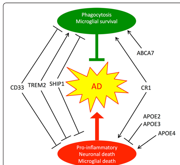
Fig. 2 Microglial activation can be neuroprotective and/or neurotoxic; the actions of AD risk proteins modulate these effects. The normal actions of CD33 and SHIP1 (encoded by INPP5D ) appear to antagonize both forms of microglial activation, while CR1 action appears to promote both A \beta phagocytosis and the production of neurotoxic pro-inflammatory cytokines such as TNF. TREM2 appears to promote phagocytosis while dampening pro-inflammatory cytokine production. ABCA7 helps to mediate phagocytosis. APOE2 and APOE3 are anti-inflammatory, while APOE4 promotes inflammation and neurotoxicity
