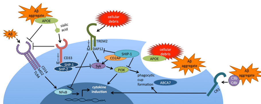
Fig. 1 Several interactions have been reported between the AD risk genes involved in inflammation. TREM2 signals through the ITAM of DAP12 to activate microglial phagocytosis; however, TREM2 expression has also been shown to dampen pro-inflammatory cytokine production activated by TLRs. Activated CD33 recruits SHP-1 and SHP-2 to inhibit Syk signaling; CD33 has also been shown to antagonize CD14/TLR4 signaling. Sialylated apoE, which complexes with A \beta , may serve as a CD33 ligand. ApoE appears to dampen TLR4 and TLR2 signaling and inhibit induction of pro-inflammatory cytokines. SHIP1 antagonizes PI3K action by converting PIP3 to PIP2; SHIP1 has also been shown to bind to and antagonize TREM2/DAP12 signaling in osteoclasts. SHIP1 also complexes with CD2AP, another AD-implicated protein, to inhibit Syk ubiquitination and degradation. CR1 is a C3b/C4b receptor that promotes phagocytosis; complement components have been shown to complex with A \beta . ABCA7 has been localized to phagocytic cups and linked to A \beta clearance, although its mechanism of action is currently unknown. Proteins encoded by genes associated with AD risk by genetics are shown with solid outlines; proteins that mediate these interactions are shown with dashed outlines
