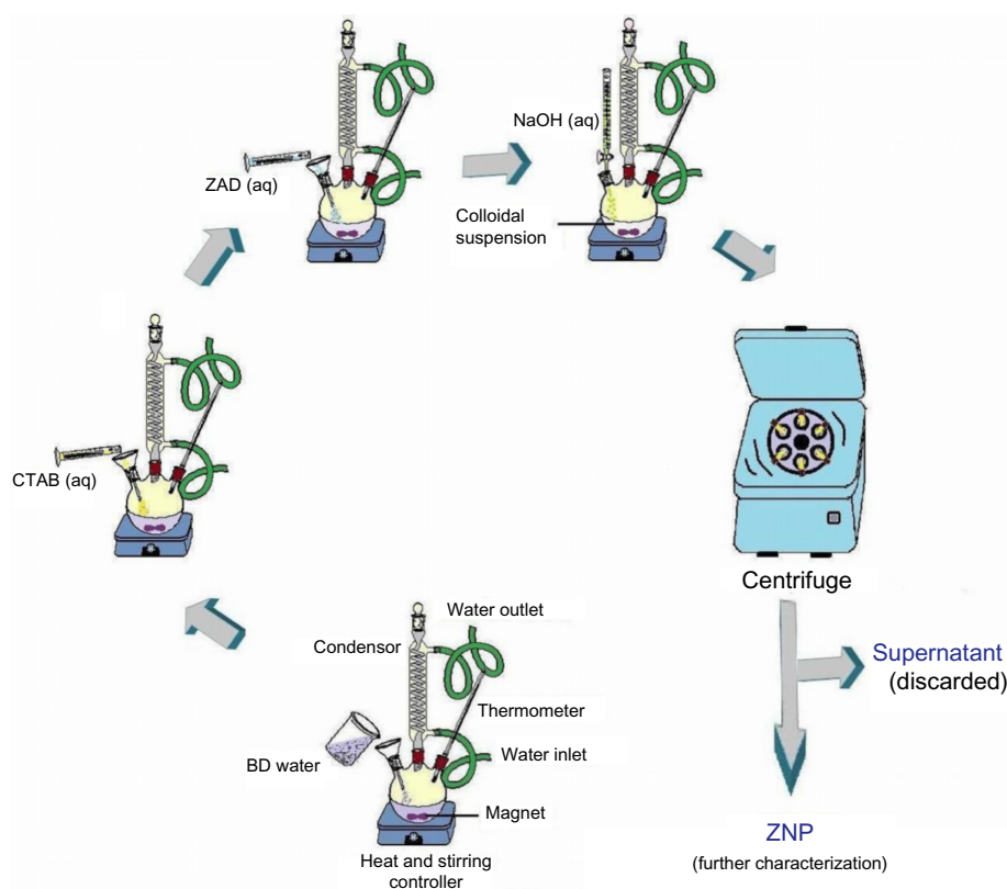
Figure 1 Flow diagram for the synthesis of ZnPs at different temperatures.
