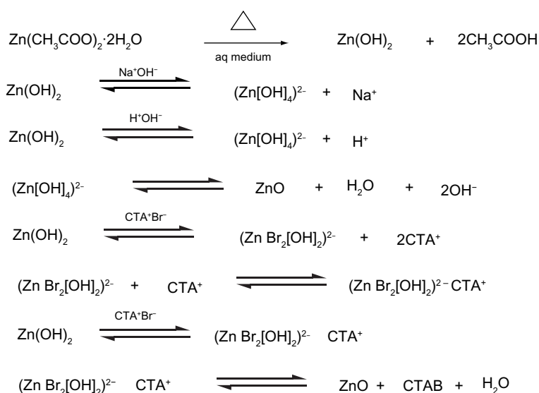
Figure 6 Reversible reactions involved in the sol–gel method of zinc oxide nanoparticle synthesis. Abbreviation: aq, aqueous.
