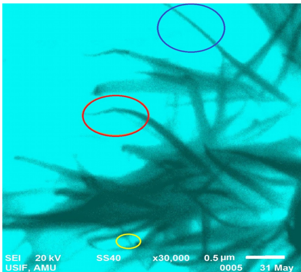
Figure 7 Growth order of the different morphologies of flower-shaped zinc oxide nanoparticle petals. Notes: Slender needle-like morphology (encircled in blue and yellow), and broad arrow-like morphology (encircled in red).
