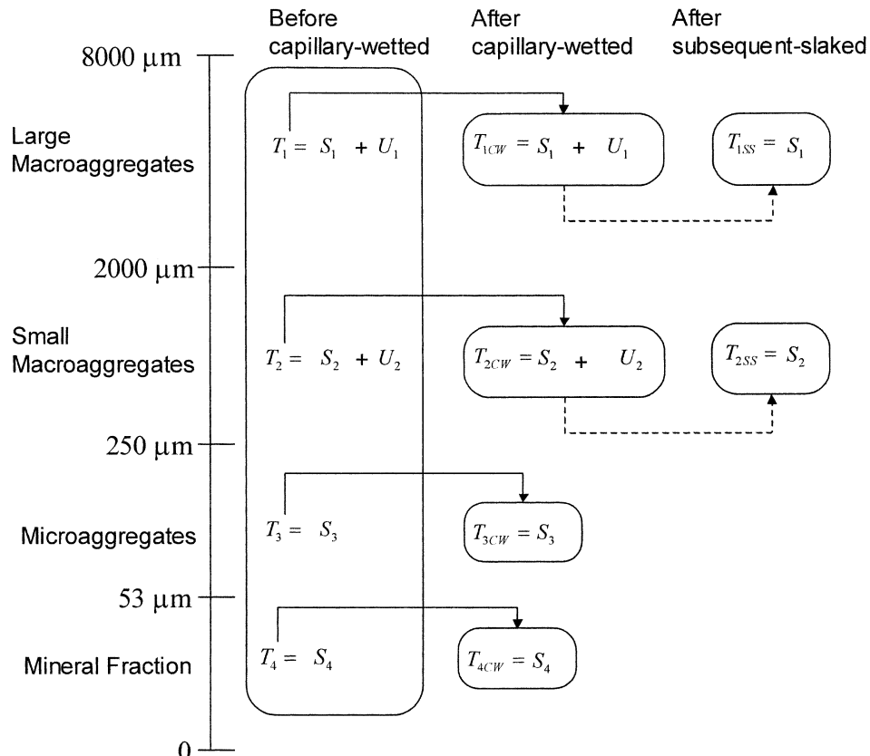
Fig. 3. General pathways involved during the capillary-wetted and the subsequent-slaked treatments. S = stable aggregates, U = unstable aggregates, T_i = total amount of aggregates in fraction i , T_{iCW} = total amount of aggregates in fraction i after capillary-wetted pretreatment, T_{iSS} = total amount of aggregates in fraction i after subsequent slaked treatment.
