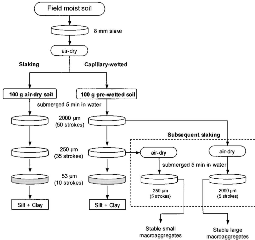
Fig. 1. Experimental procedure used to assess aggregate-size stability distribution.
