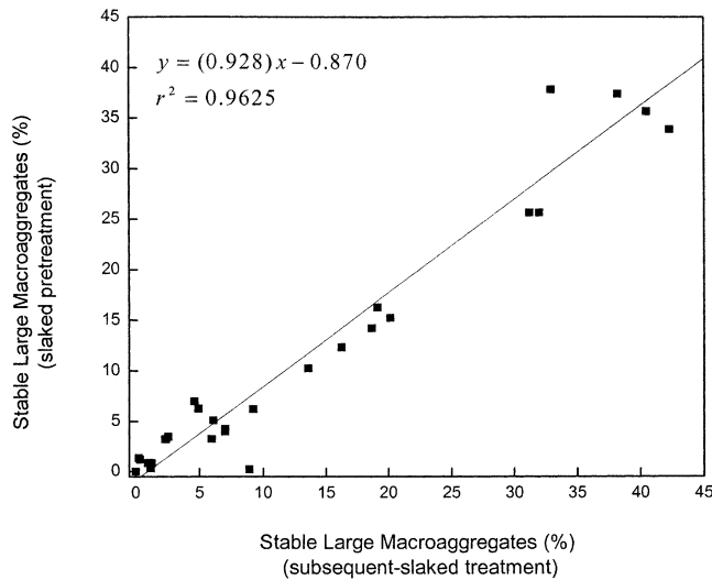
Fig. 4. Relationship between the mass of large macroaggregates >2000 \mu\text{m} quantified by slaked pretreatment ( T_{1s} ) and stable large macroaggregates >2000 \mu\text{m} quantified by the subsequent-slaking treatment ( T_{1ss} ). Values are expressed as percentages of soil dry and on a sand-free basis.
