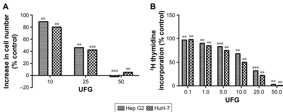
Figure 3 Effect of the UFG-PLGA-NP on Hep G2 and HuH-7 cell lines.
