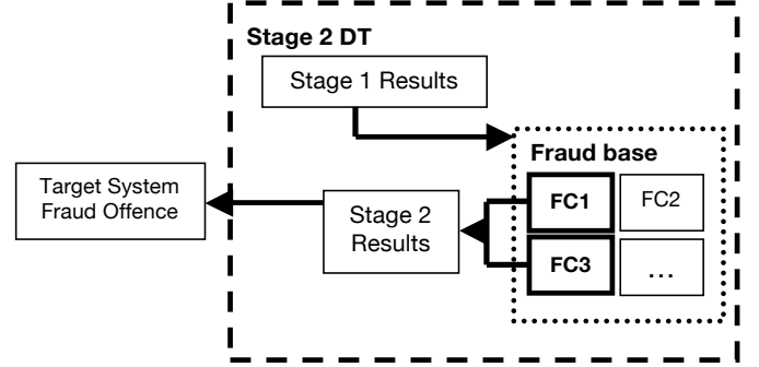
Figure 3: Structure of the CBR-FT framework for Stage 2. The cases FC_1 and FC_3 are those cases in the knowledge base with locations matching those found in the current investigation during Stage 1. These locations are analysed to identify a further set of lower-priority locations of possible evidence.
