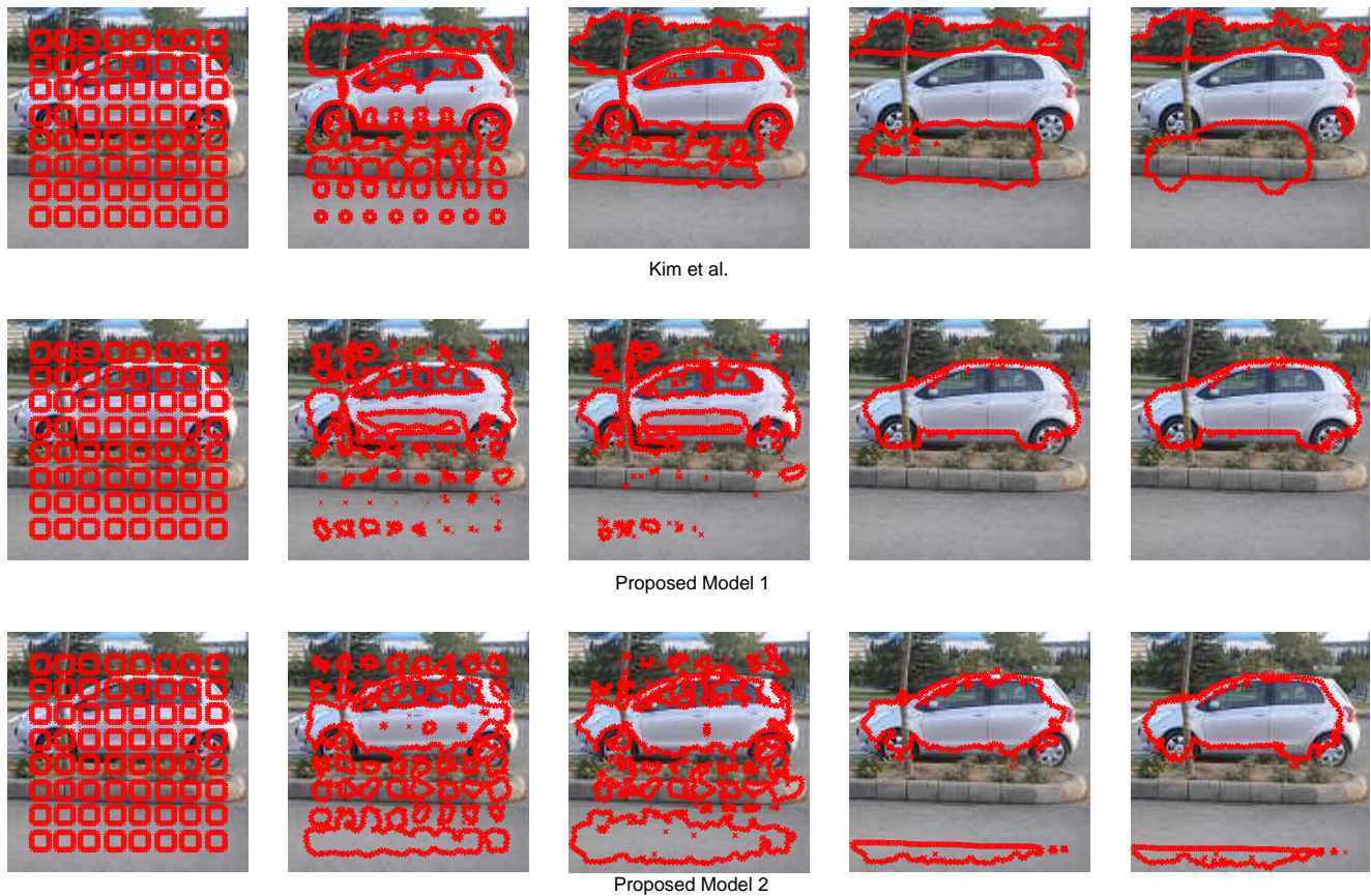
Fig. 10 Segmentation of a car. First row shows the segmentation result of [12]. Second row shows the segmentation result of proposed model 1. Third row shows the result of proposed model 2. Leftmost and rightmost columns show the initial curve and the final segmentation result, respectively, whereas the middle columns show intermediate states in the curve evolution process.
