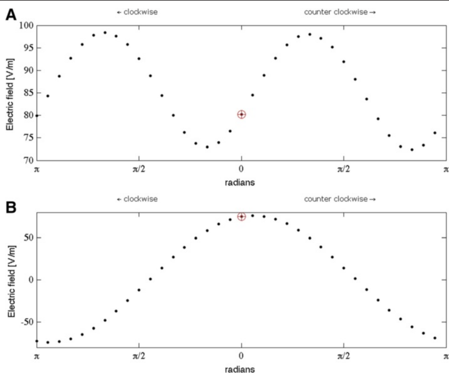
Figure 4 Mean electric field strength in target region M1: The mean electric field values for (A) |\vec{E}| and (B) E_{\perp} within the target region M1. The standard coil orientation from literature is indicated separately in both panels (red circle with cross). The coil is rotated in steps of 10 degrees.
