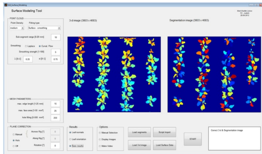
Figure 7 GUI for surface modeling. Graphical user interface for surface modeling: Disparity data (left) and segmentation data (right) are combined in module 3 to approximate surfaces to 3-d point clouds according to different modeling options. Surfaces are either fitted according to planar, quadratic or cubic functions or smoothed using curvature flow or Laplace smoothing.
