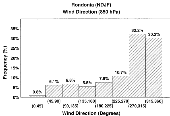
FIG. 4. Frequency distribution of wind direction (850 hPa) in the reference region in Rondônia. Wind direction is counted clockwise (in degrees) from the north. Period: 1 Nov–28 Feb 1980–99.
