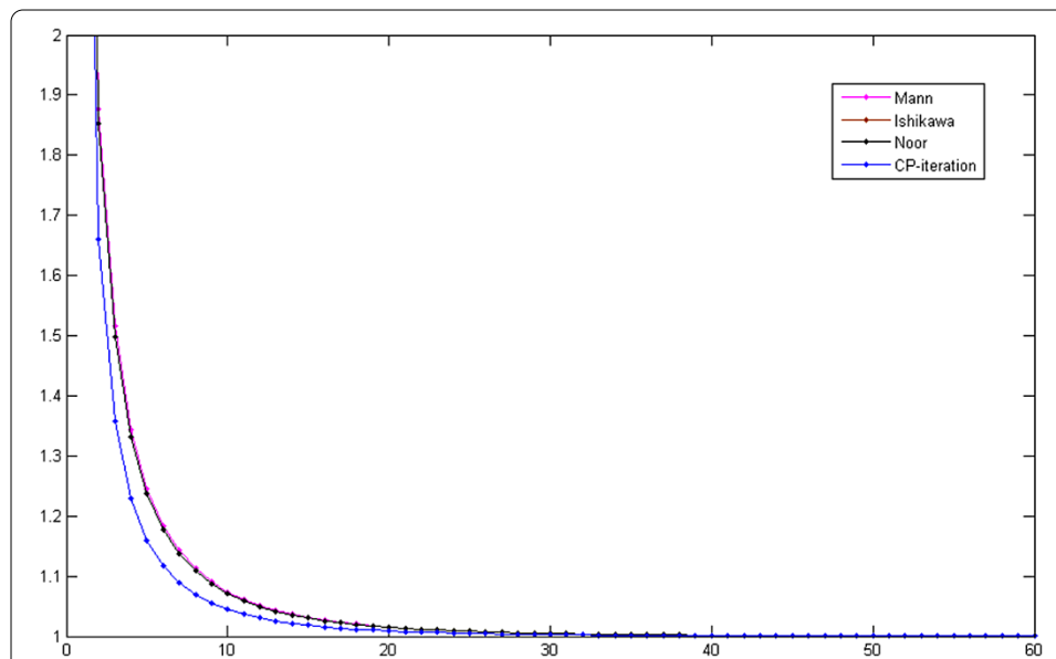
Figure 1 Convergence behavior of Mann, Ishikawa, Noor and CP iterations for the function given in Example 3.1.
