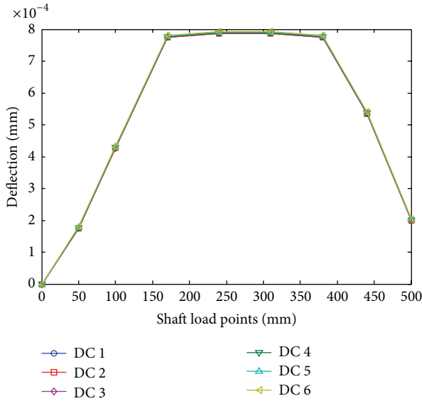
FIGURE 2: Comprehensive deflection cycles analysis.
