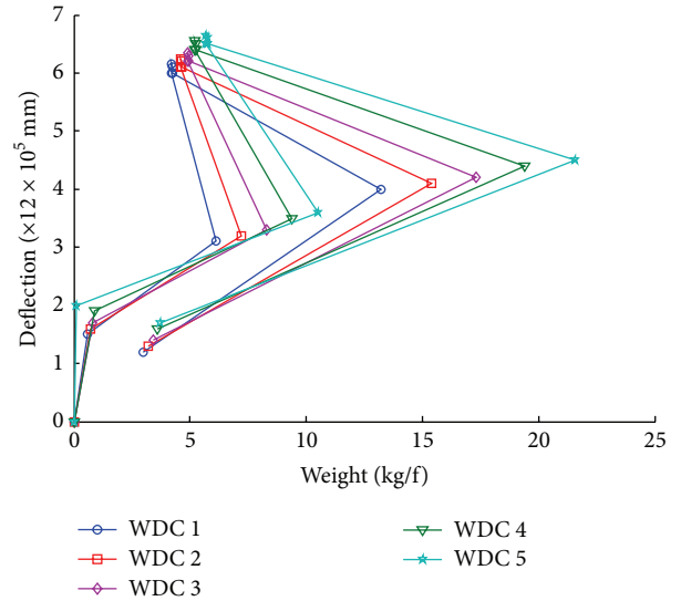
FIGURE 5: Graph of weight versus deflection cycles analysis.
