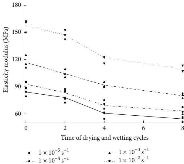
FIGURE 5: Elastic modulus of CA mortar.
