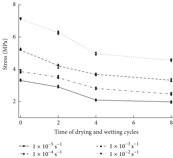
FIGURE 4: Compressive strength of CA mortar at different strain rates and drying and wetting cycle times.
