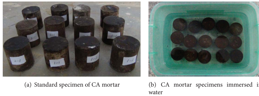
FIGURE 1: CA mortar specimens.
