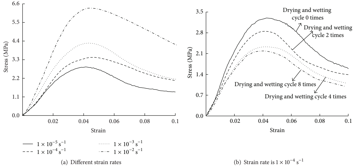
FIGURE 3: Stress-strain full curves of CA mortar.
