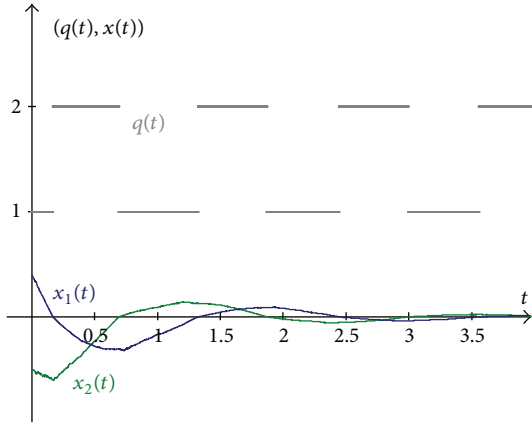
FIGURE 5: Simulation of the hybrid system (53) with stabilizing switching \sigma = \sigma_{st} for p = 1 .
