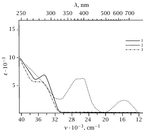
Figure 2. Transformation of the absorption spectrum of the compound (I) in ethanol at 77 K. 1-before the irradiation, 2-after the irradiation ( T = 77 \text{ K} , \lambda_{\text{exc}} = 313 \text{ nm} , \tau_{\text{exc}} = 15 \text{ min} ), 3-AFTER defreezing ( T = 293 \text{ K} ).
