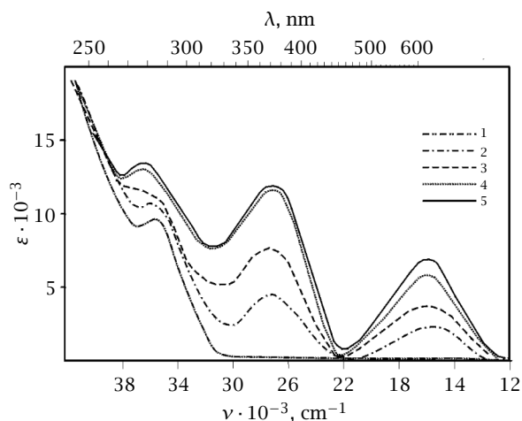
Figure 1. Transformation of the absorption spectrum of the compound (I) under irradiation in ethanol, T = 293 \text{ K} , \lambda_{\text{exc}} = 313 \text{ nm} . Curves 1,2,3,4 correspond to the time of irradiation-0,8,13,40 mins.5-the absorption spectrum of the phenoxazinone (II).
