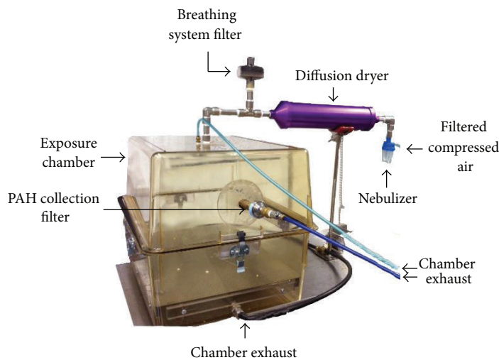
FIGURE 2: PAH chamber. Mice were exposed to PAH or normal air in two side-by-side chambers delivered via aerosol (only one shown). Filters were collected as depicted and used to measure ambient concentrations.
