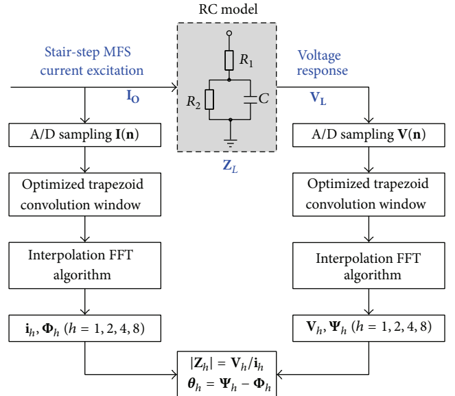
FIGURE 7: Impedance measurement scheme.
