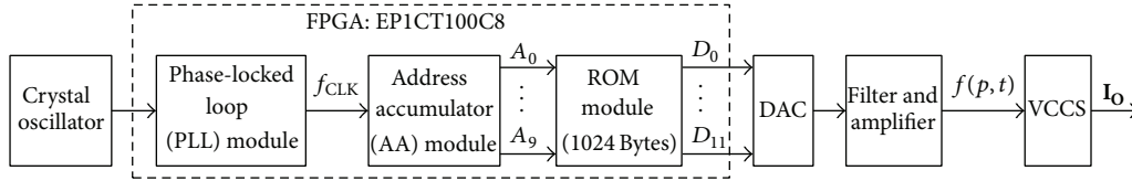
FIGURE 5: Block diagram of the hardware system to realize the MFS signal.
