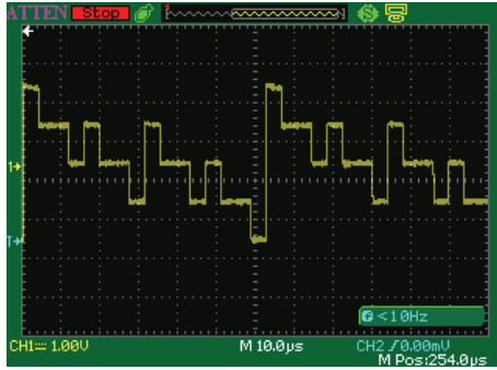
FIGURE 6: Oscillograph of f(4, t) (one more period).
