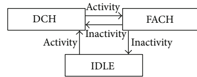
FIGURE 3: Simplified Radio Resource Control state model.
